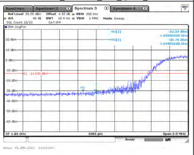
LTE Band 2_CH18675_15M_QPSK_Full RB
