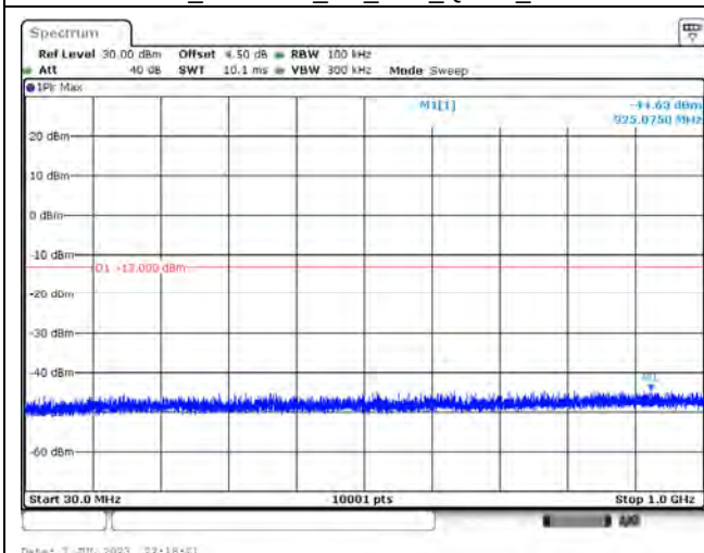
LTE Band 7_CH21425_5M_1RB_QPSK_Below 1GHz
