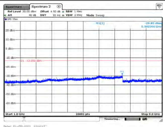
LTE Band 5_CH20635_3M_1RB_QPSK_Above 1GHz
