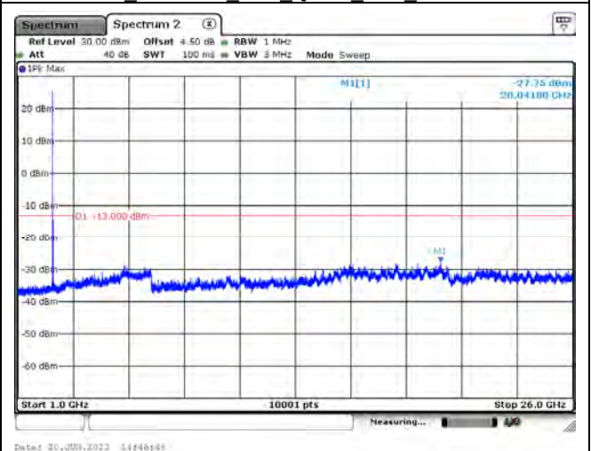
LTE Band 7_CH21400_10M_QPSK_1RB_Above 1GHz
