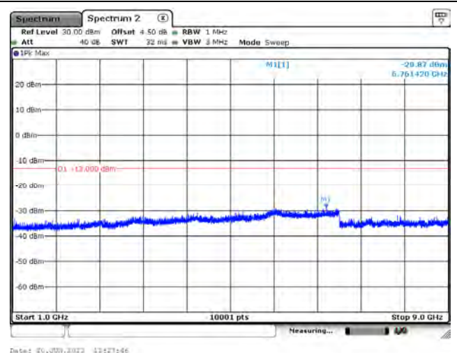
LTE Band 5_CH20600_10M_1RB_QPSK_Above 1GHz
