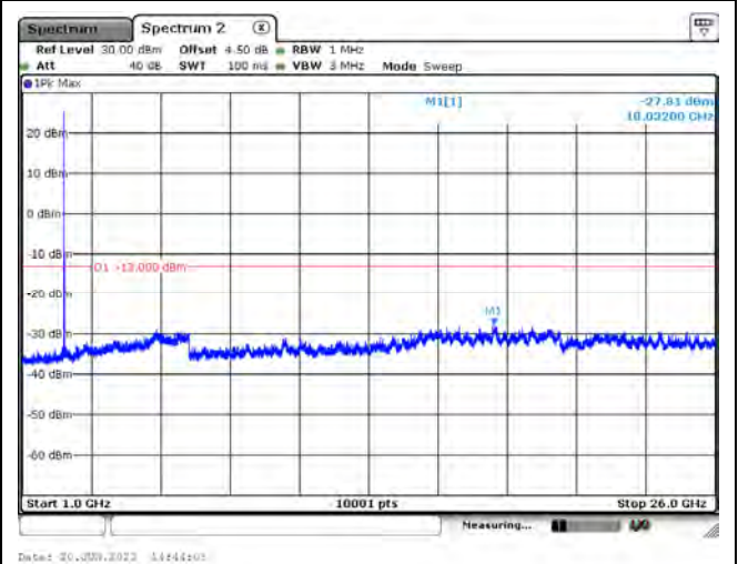
LTE Band 7_CH21100_10M_QPSK_1RB_Above 1GHz
