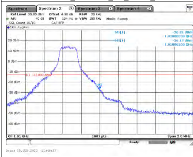
LTE Band 2_CH19175_5M_QPSK_1RB
