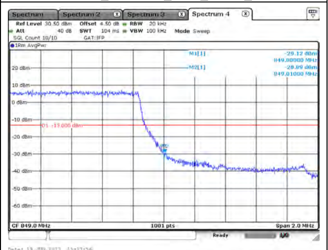
LTE Band 5_CH20643_1.4M_QPSK_Full RB
