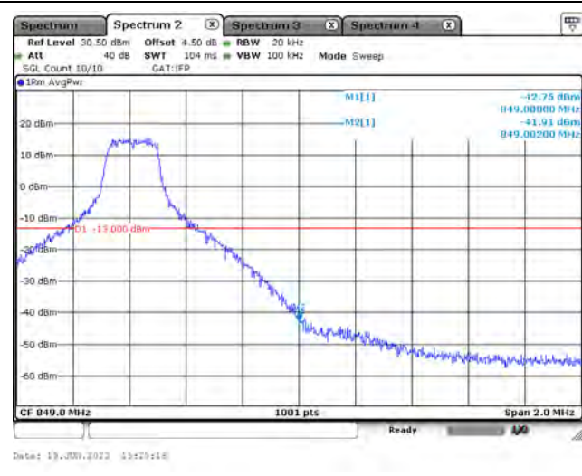
LTE Band 5_CH20600_10M_QPSK_1RB
