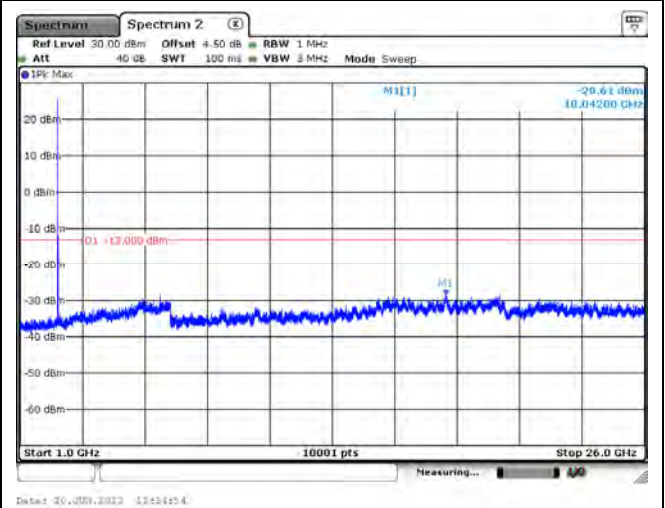
LTE Band 7_CH21100_5M_1RB_QPSK_Above 1GHz
