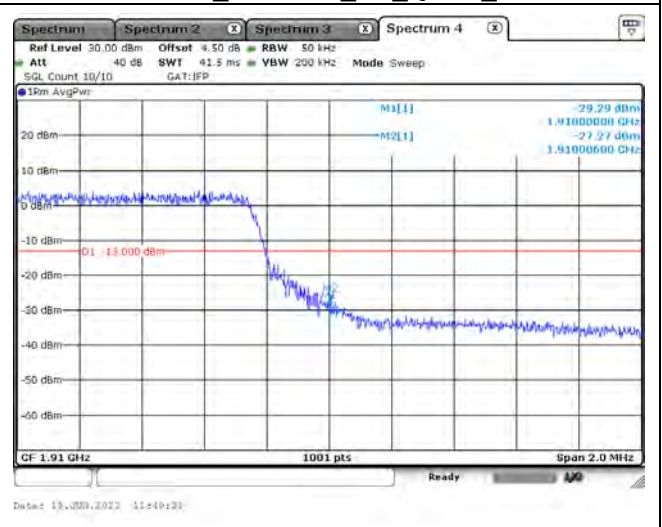
LTE Band 2_CH19175_5M_QPSK_Full RB
