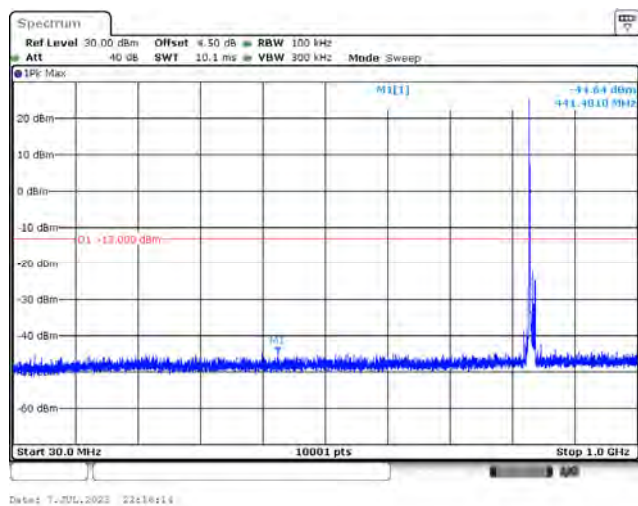
LTE Band 5_CH20600_10M_1RB_QPSK_Below 1GHz
