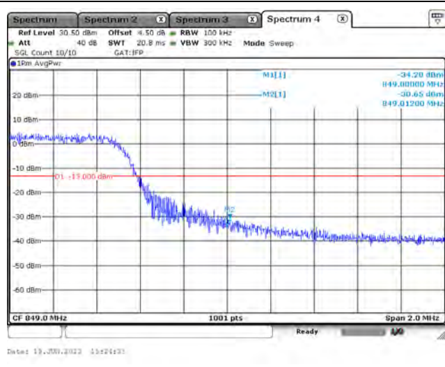
LTE Band 5_CH20600_10M_QPSK_Full RB
