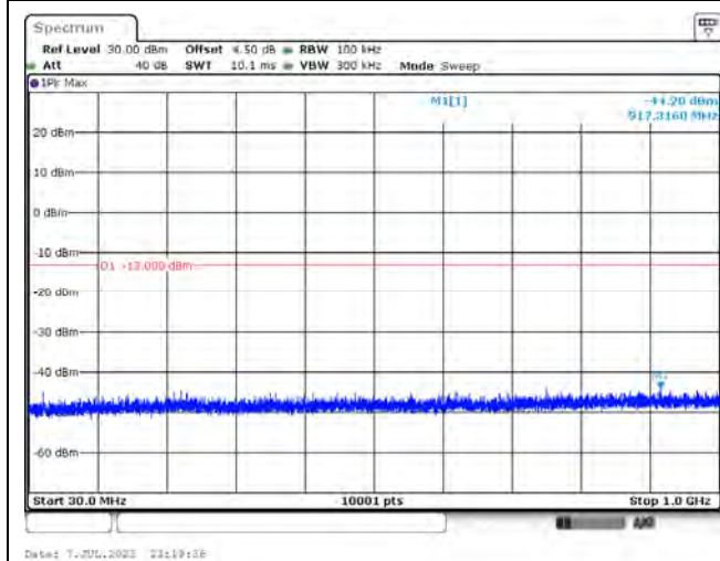
LTE Band 7_CH21100_10M_QPSK_1RB_Below 1GHz
