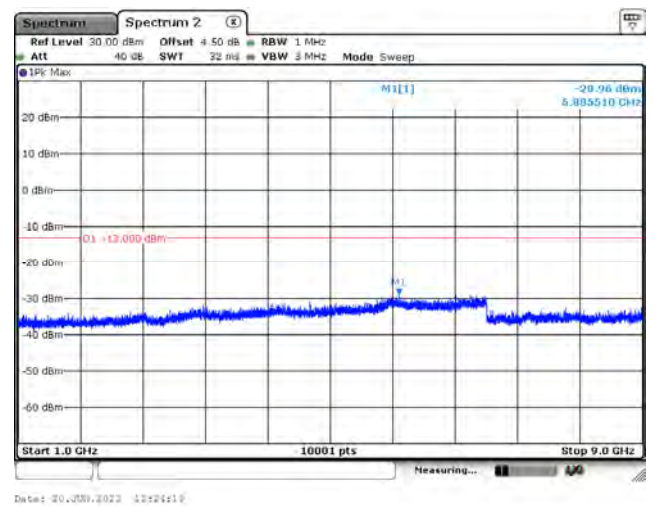
LTE Band 5_CH20525_10M_1RB_QPSK_Above 1GHz
