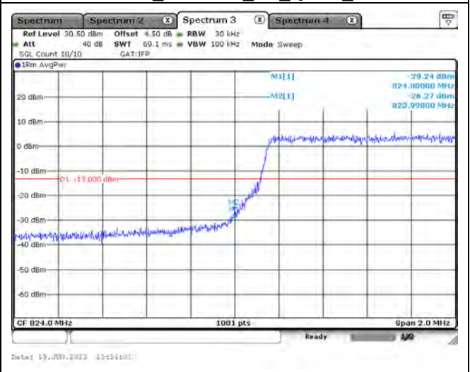
LTE Band 5_CH20415_3M_QPSK_Full RB
