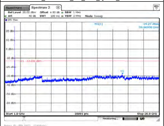
LTE Band 7_CH21425_5M_1RB_QPSK_Above 1GHz
