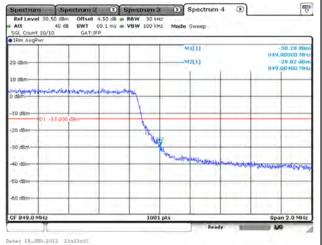
LTE Band 5_CH20425_5M_QPSK_Full RB
