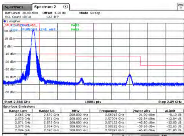
LTE Band 7_CH21375_15M_QPSK_1RB
