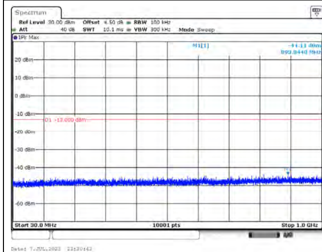
LTE Band 7_CH21400_10M_QPSK_1RB_Below 1GHz
