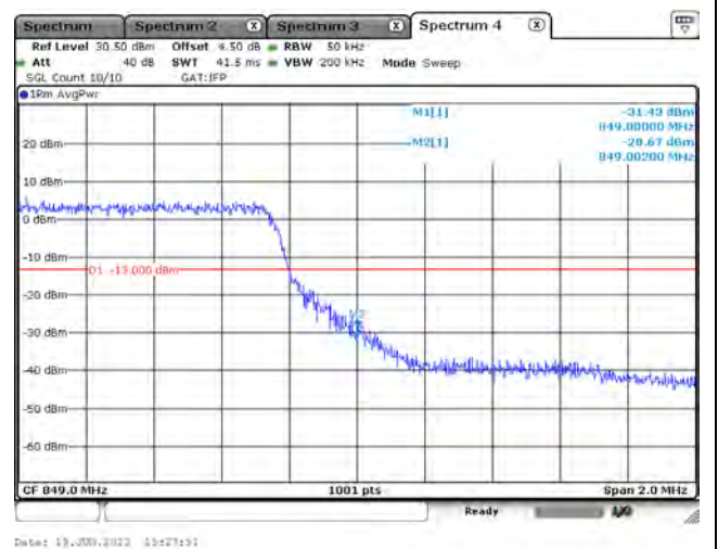
LTE Band 5_CH20625_5M_QPSK_Full RB
