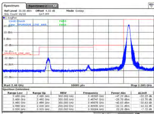
LTE Band 7_CH20825_15M_QPSK_1RB
