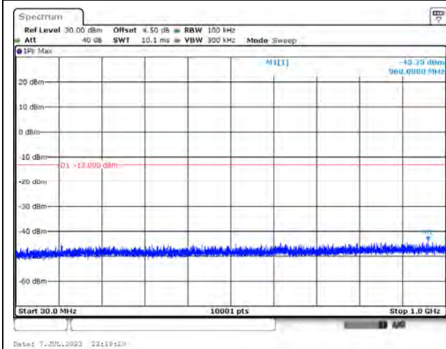
LTE Band 7_CH21100_5M_1RB_QPSK_Below 1GHz
