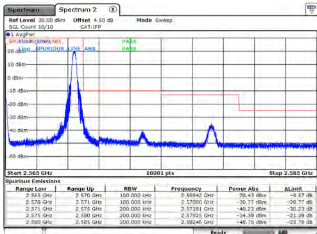
LTE Band 7_CH21400_10M_QPSK_1RB
