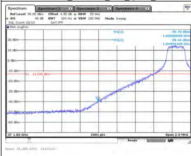
LTE Band 2_CH18675_15M_QPSK_1RB
