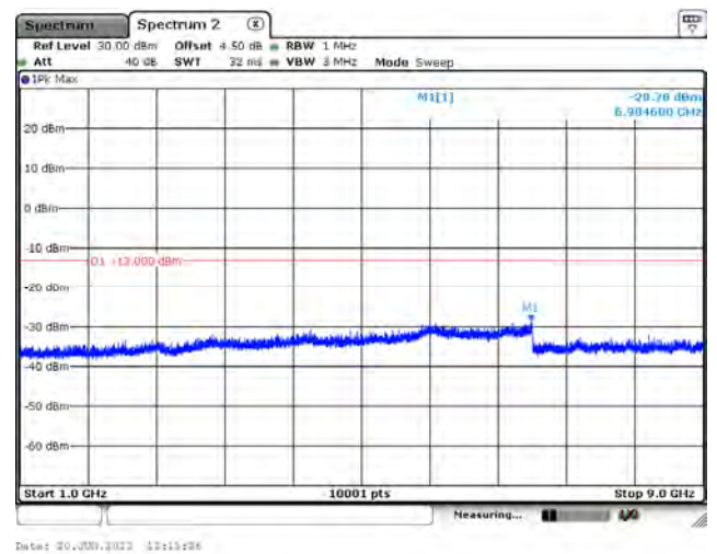
LTE Band 5_CH20525_3M_1RB_QPSK_Above 1GHz
