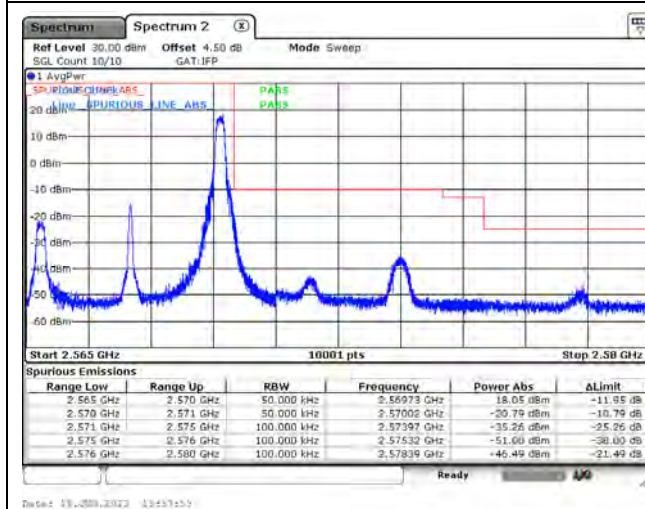
LTE Band 7_CH20800_10M_QPSK_1RB
