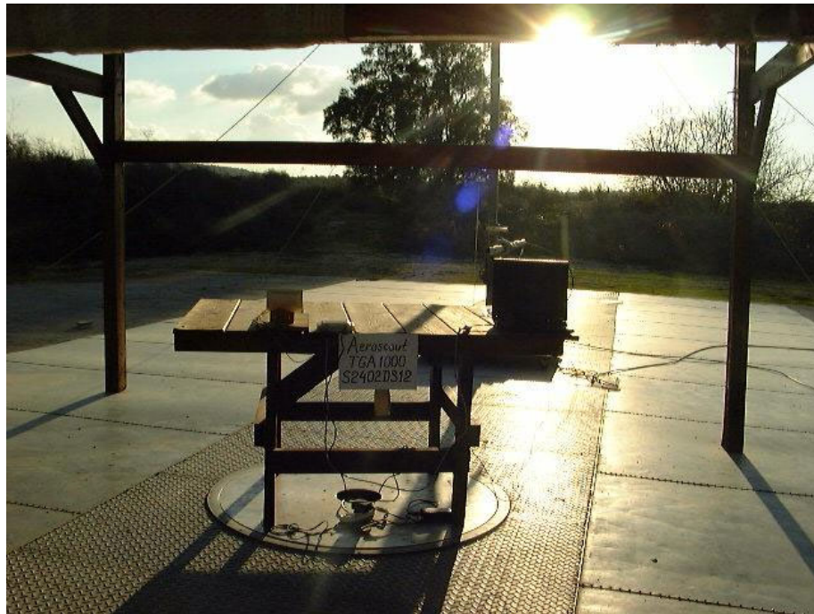
Figure 5. Spurious Radiated Emission Test Antenna S2402DS12
