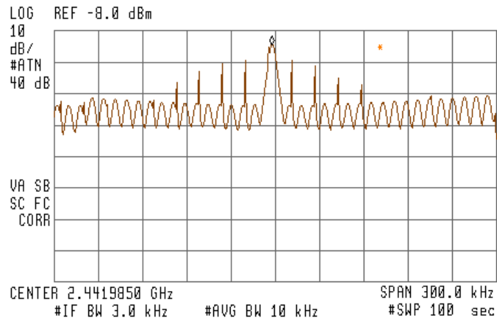
Figure 61 —2442 MHz
