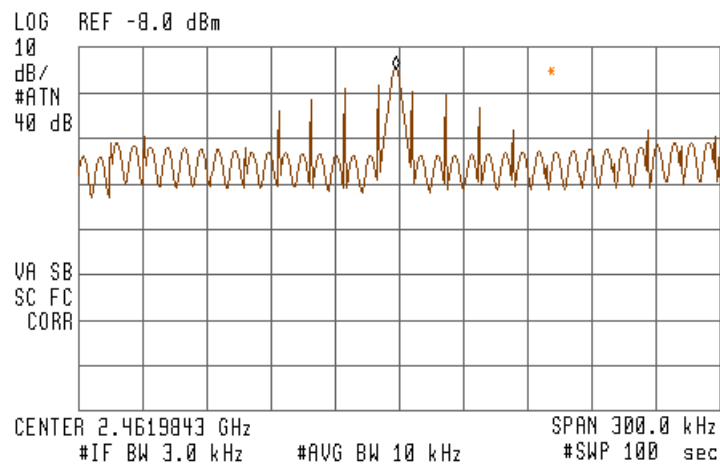
Figure 62 —2462 MHz
