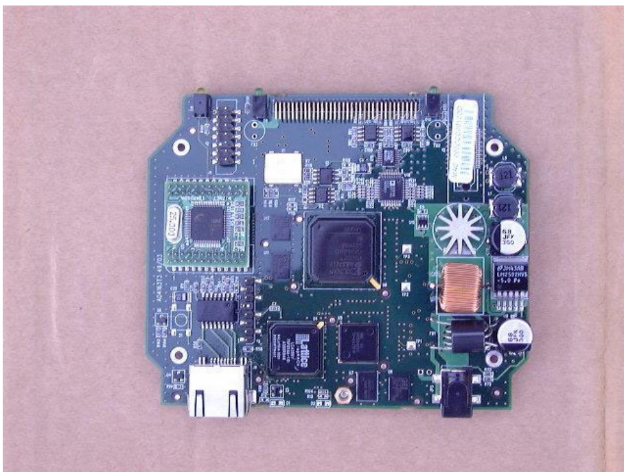
Figure 9 PCB 2 Side 1
