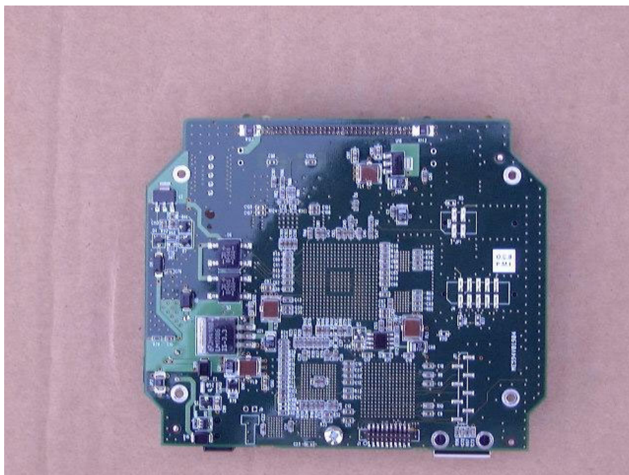
Figure 10 PCB 2 Side 2
