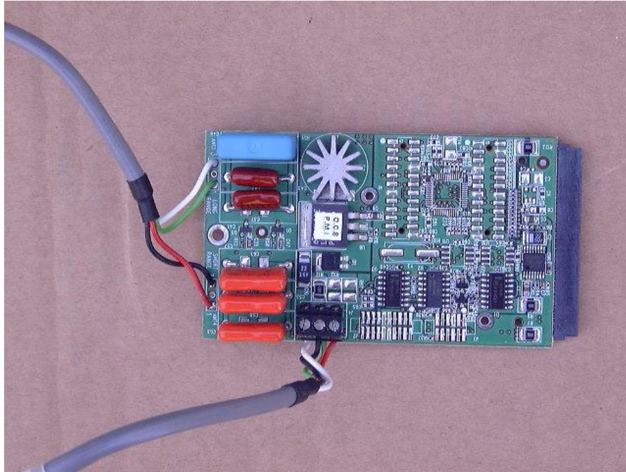
Figure 7 PCB 1 Side 1
