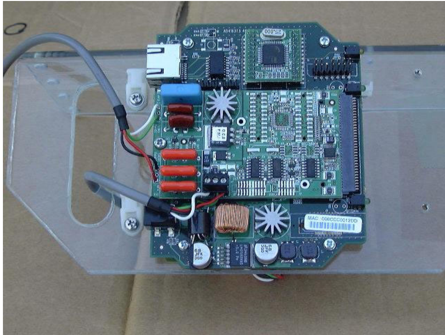
Figure 5 PCBs Side 2
