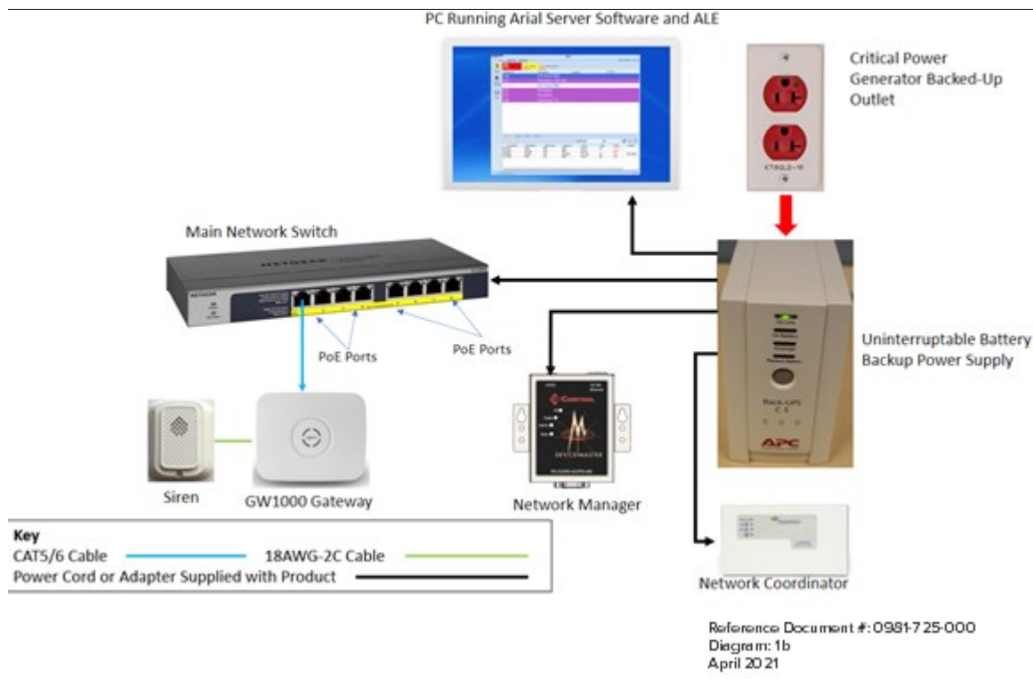
Figure 2. Arial 900 System Power Connection Overview
