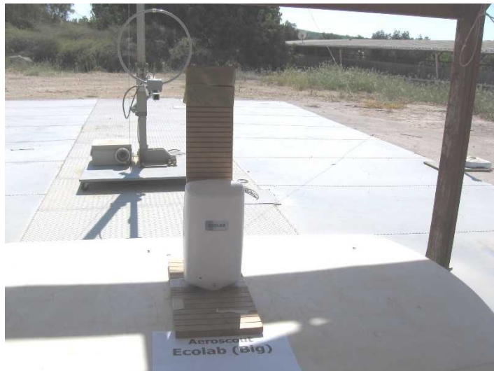
Radiated Emission Test – M/N: 92021188 (Ecolab NEXA big)
