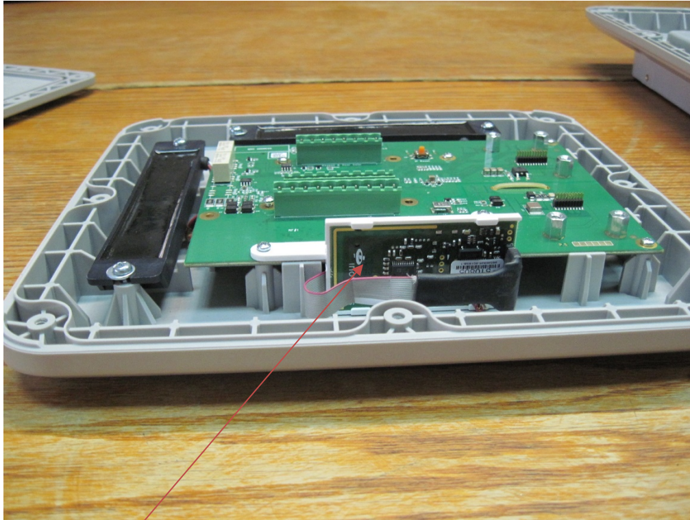
Inovonics card
