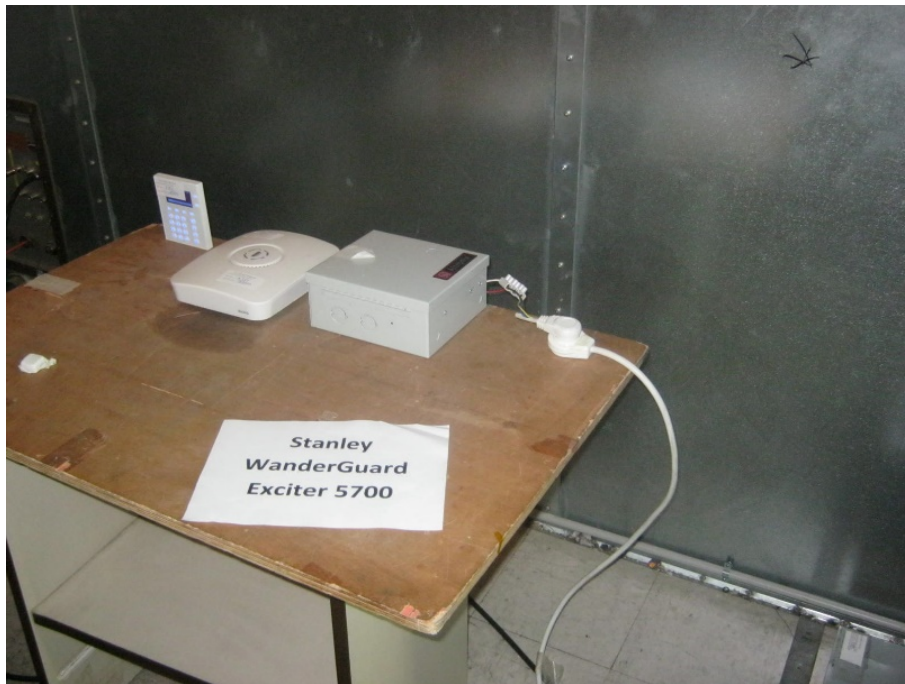
Conducted Emission from AC Mains (AC/DC adapter type 1) Test Setup
