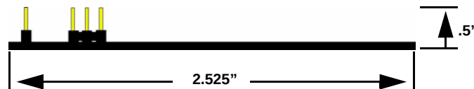
Figure 4 E*1941 One-Way Serial RF Module Dimensions
