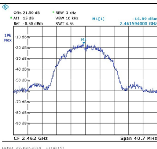
Figure 68. 2462.0 MHz, Wi-fi/b(11Mbit/s)
