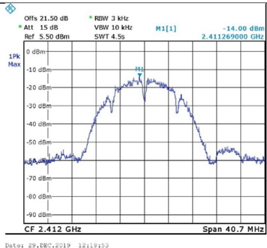
Figure 65. 2412.0 MHz, Wi-fi/b(1Mbit/s)
