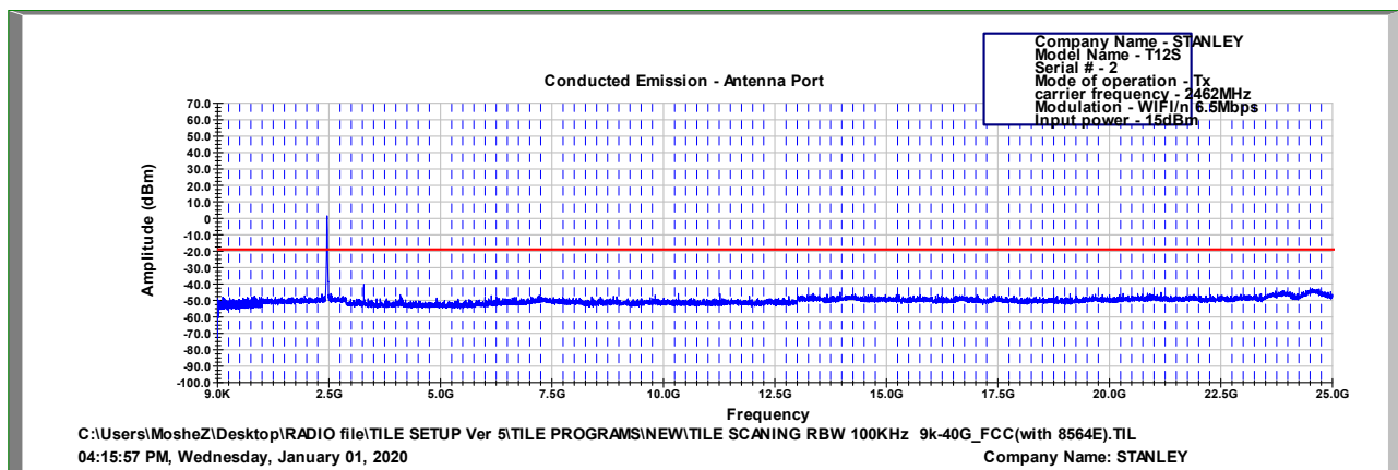
Figure 117 2462.0 MHz, WI-FI/n(6.5Mbit/s)
