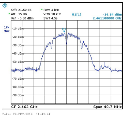
Figure 69. 2462.0 MHz, Wi-fi/b(1Mbit/s)
