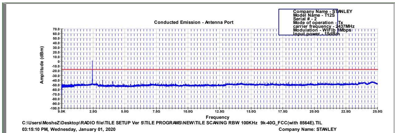
Figure 104 2437.0 MHz, WI-FI/b(1Mbit/s)
