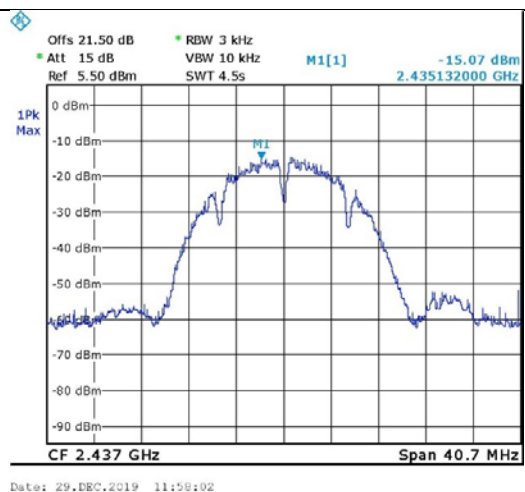
Figure 67. 2437.0 MHz, Wi-fi/b(1Mbit/s)
