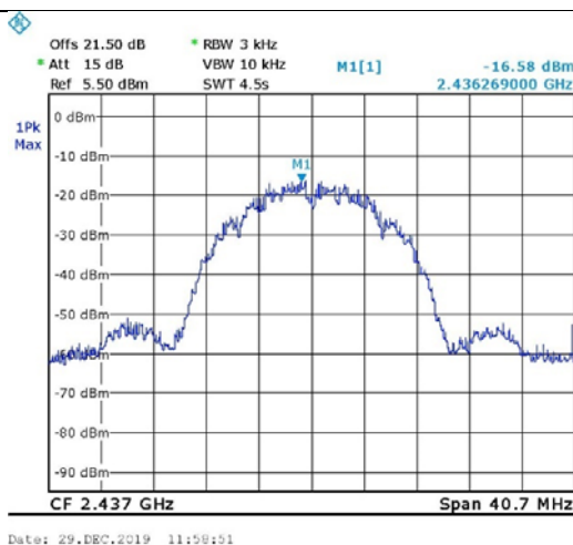
Figure 66. 2437.0 MHz, Wi-fi/b(11Mbit/s)
