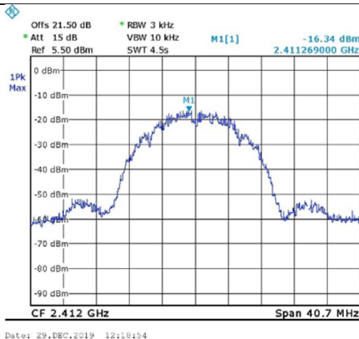
Figure 64. 2412.0 MHz, Wi-fi/b(11Mbit/s)
