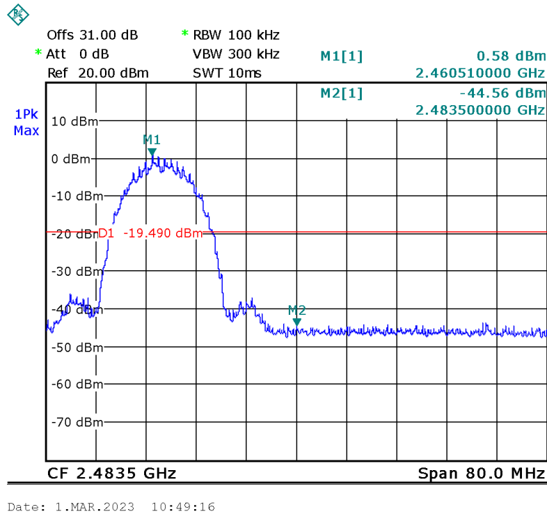
Figure 61. 2462.0 MHz, Wi-fi/b (11Mbit/s)
