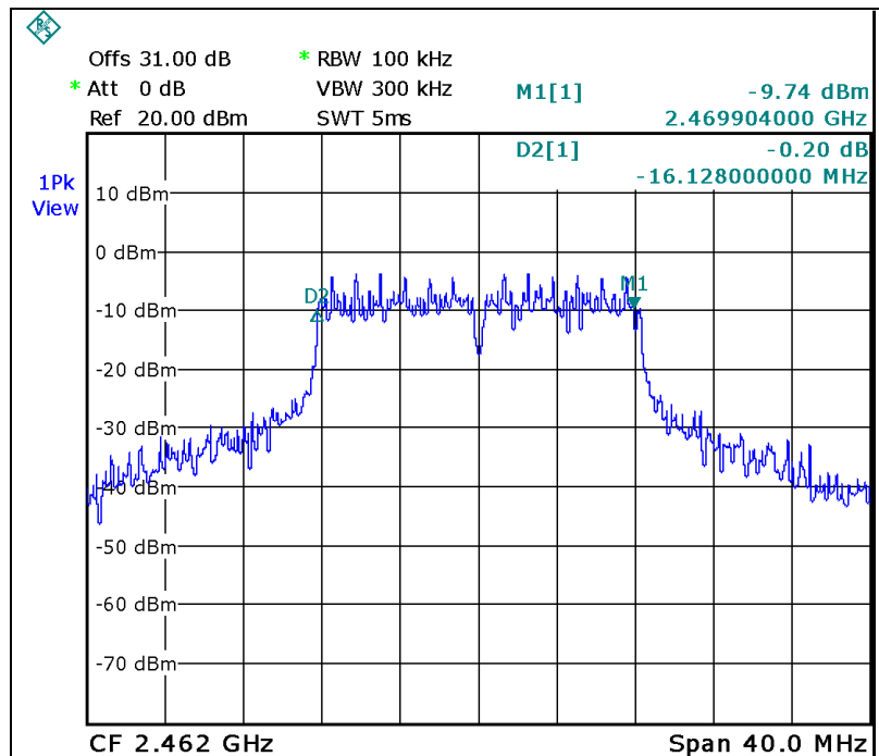
Figure 13. 2462.0 MHz, Wi-fi/g (54Mbit/s)
