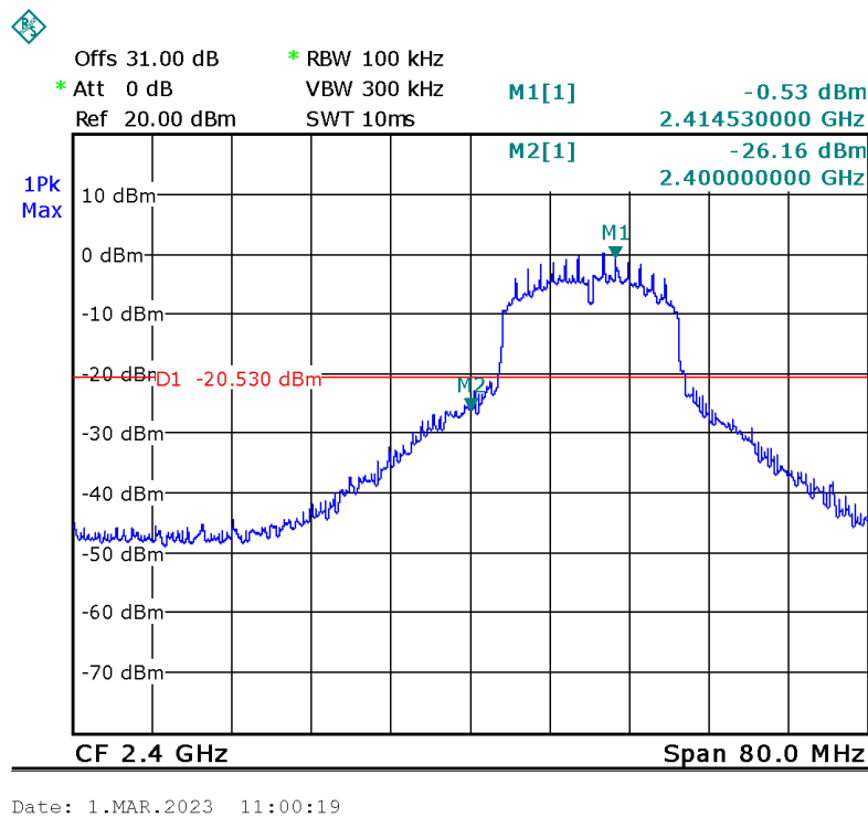
Figure 62. 2412.0 MHz, Wi-fi/n (6.5Mbit/s)
