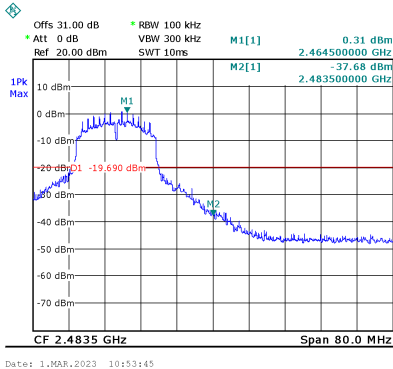
Figure 63. 2462.0 MHz, Wi-fi/n (6.5Mbit/s)
