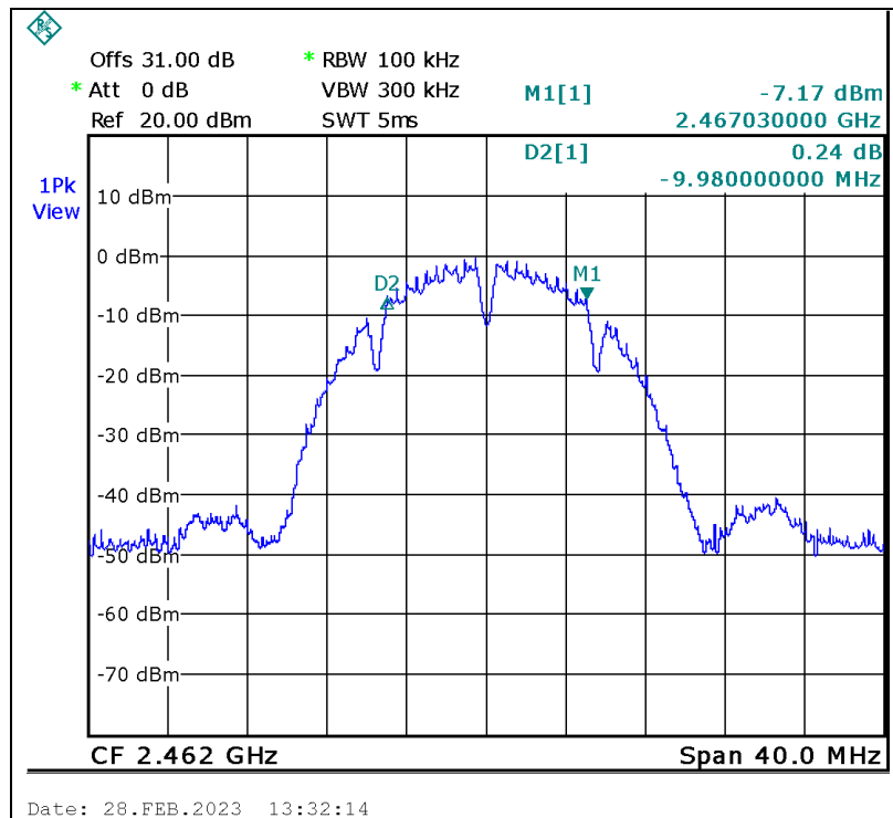
Figure 17. 2462.0 MHz, Wi-fi/b (1Mbit/s)
