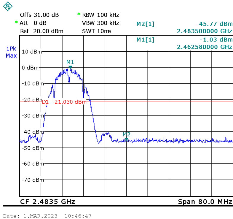
Figure 59. 2462.0 MHz, Wi-fi/b (1Mbit/s)
