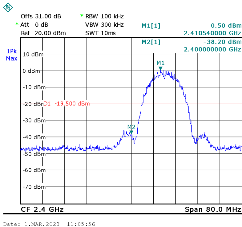
Figure 60. 2412.0 MHz, Wi-fi/b (11Mbit/s)
