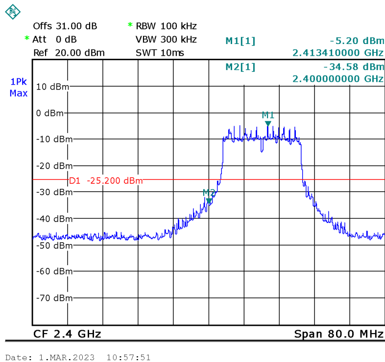
Figure 64. 2412.0 MHz, Wi-fi/n (65Mbit/s)
