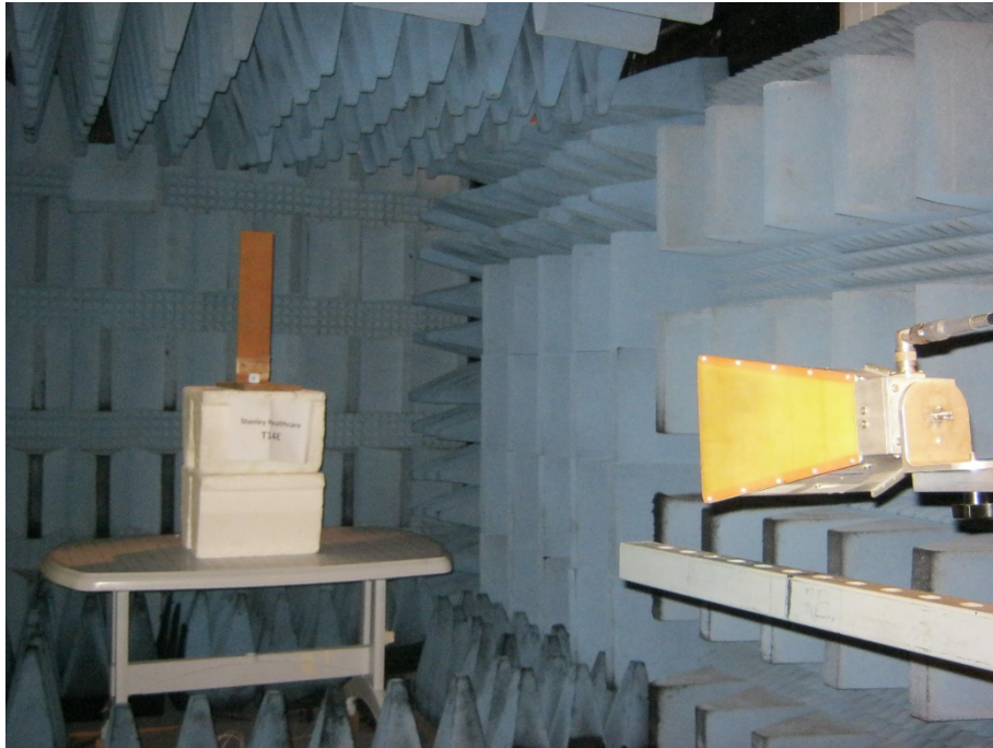
Radiated Emission Test, 1000-18,000MHz
