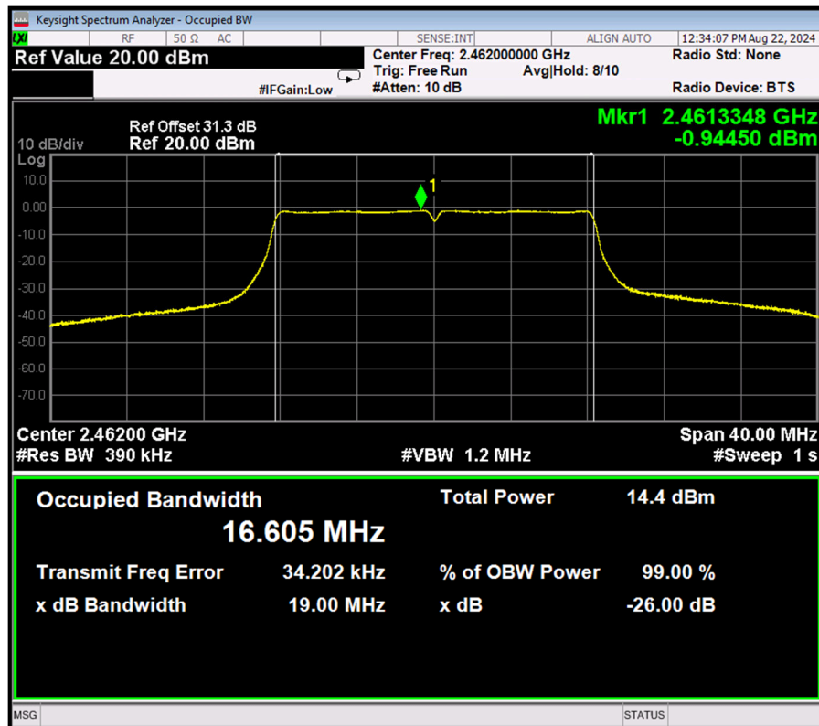
Figure 100. 2462.0 MHz, Wi-fi/g(6Mbit/s)
