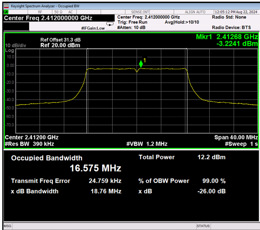
Figure 97. 2412.0 MHz, Wi-fi/g(54Mbit/s)
