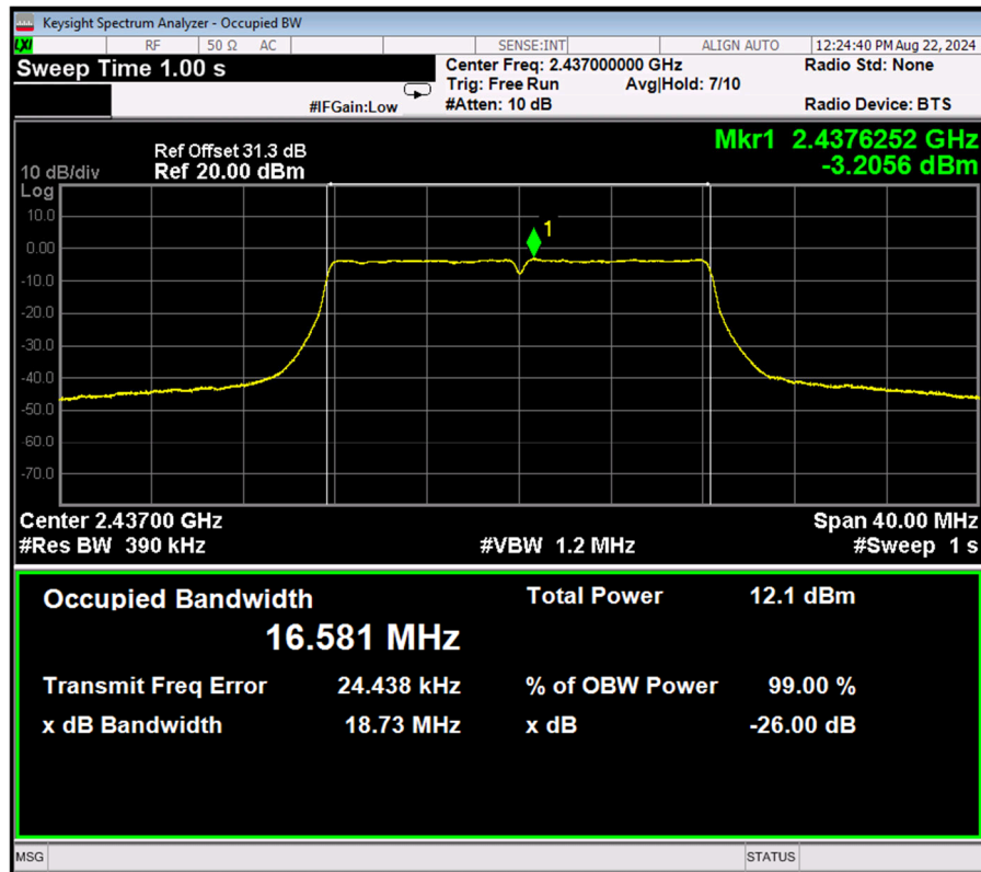
Figure 99. 2437.0 MHz, Wi-fi/g(54Mbit/s)
