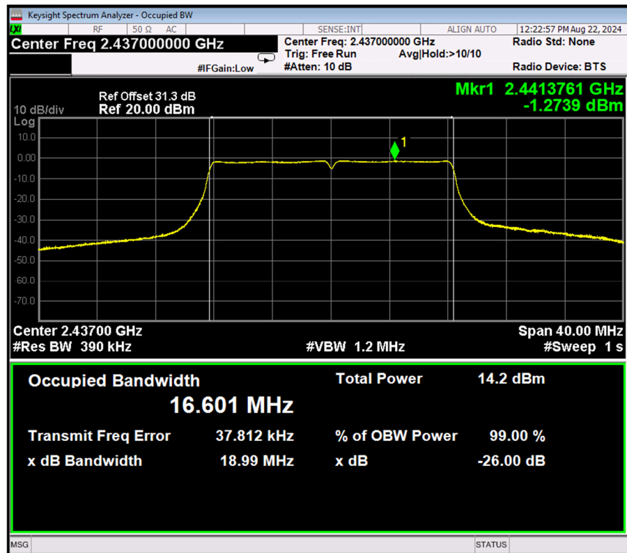
Figure 98. 2437.0 MHz, Wi-fi/g(6Mbit/s)
