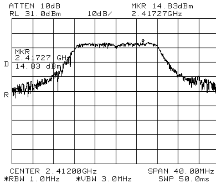
Figure 44. 2412 MHz, OFDM (4 QAM) Modulation
