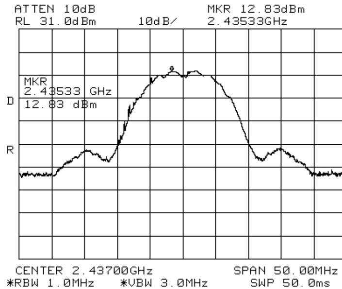
Figure 42. 2437 MHz, DSSS Modulation
