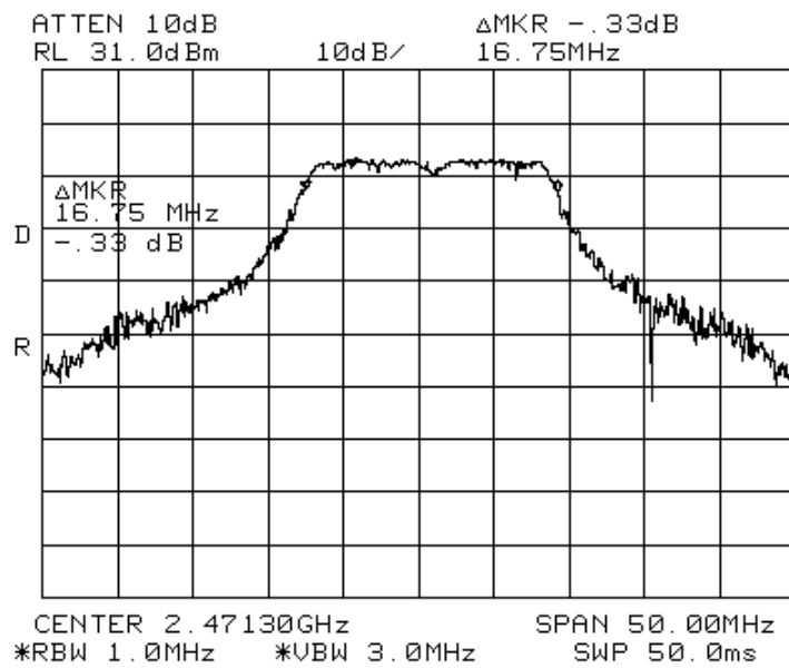
Figure 21. 2472 MHz, OFDM (BPSK) Modulation
