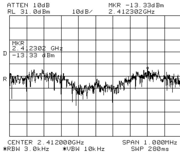
Figure 77. 2412 MHz, OFDM (4 QAM) Modulation
