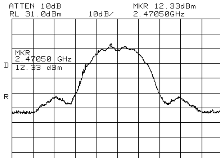
Figure 43. 2472 MHz, DSSS Modulation
