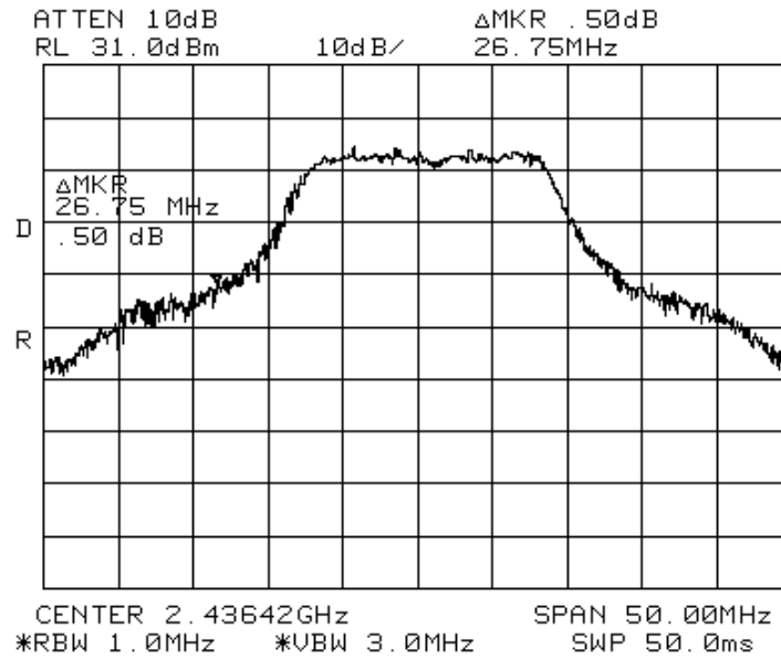
Figure 34. 2437 MHz, OFDM (16 QAM) Modulation
