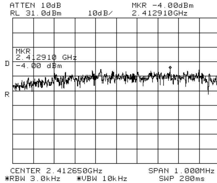
Figure 74. 2412 MHz, DSSS Modulation
