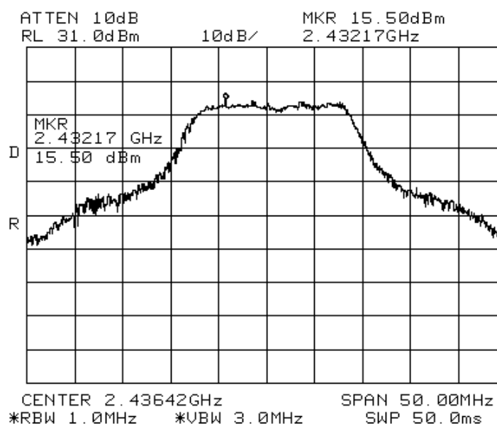
Figure 51. 2437 MHz, OFDM (16 QAM) Modulation
