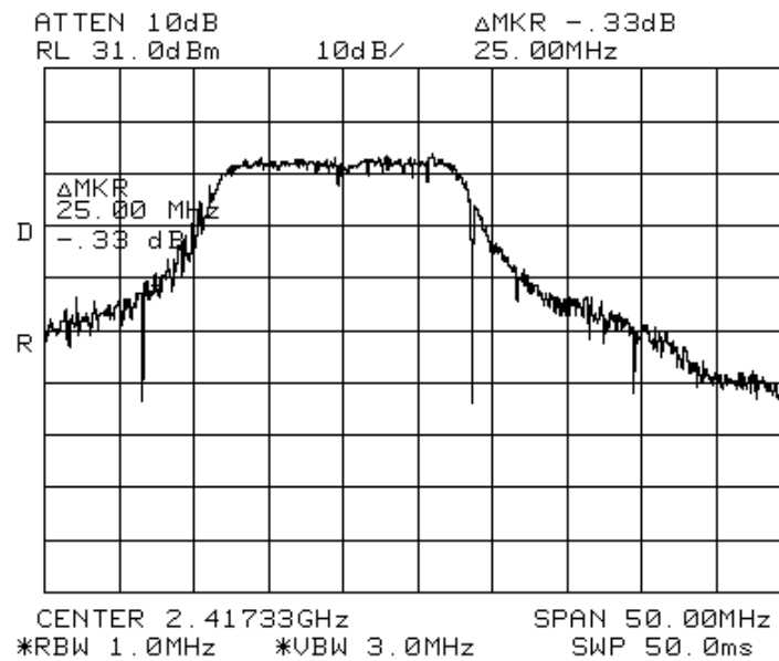
Figure 33. 2412 MHz, OFDM (16 QAM) Modulation
