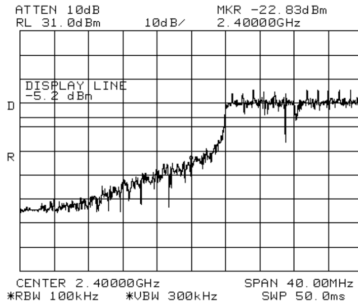
Figure 60 —Lower Band Edge, OFDM (4 QAM) Modulation
