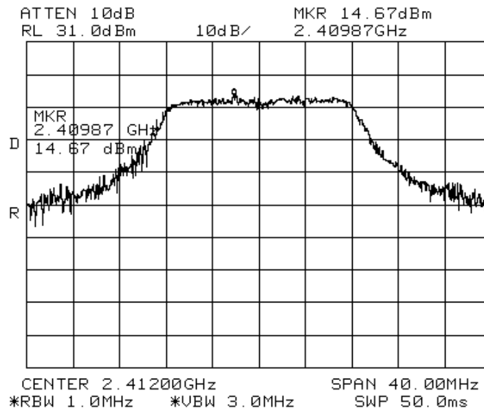
Figure 50. 2412 MHz, OFDM (16 QAM) Modulation
