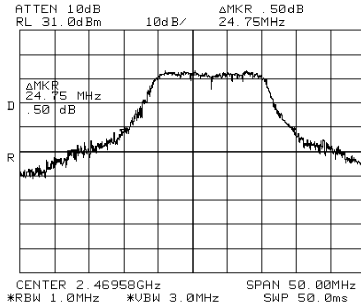
Figure 32. 2472 MHz, OFDM (64 QAM) Modulation
