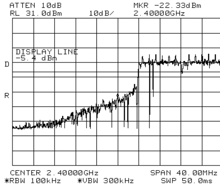
Figure 64 —Lower Band Edge, OFDM (16 QAM) Modulation
