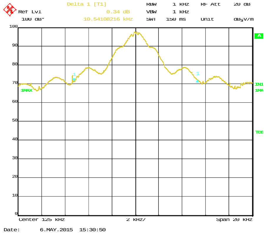
Figure 11. 26dB Bandwidth
