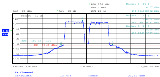
Figure 8.8-4: Conducted band edge and adjacent channel emissions sample plot for multi 6 MHz channel
