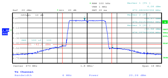
Figure 8.7-1: PSD within 100 kHz and Power within 6 MHz sample plot for single 6 MHz channel
