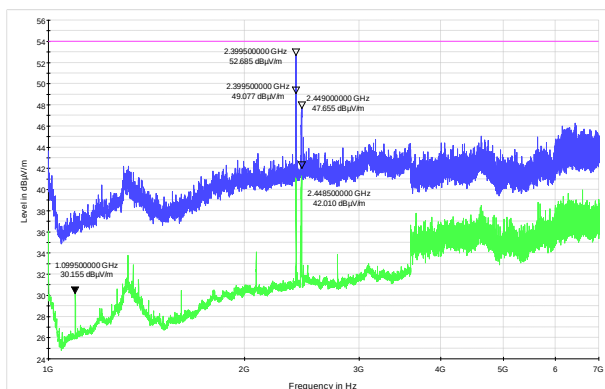
Figure 8.9-9: Radiated spurious emissions within 1–7 GHz for high channel
