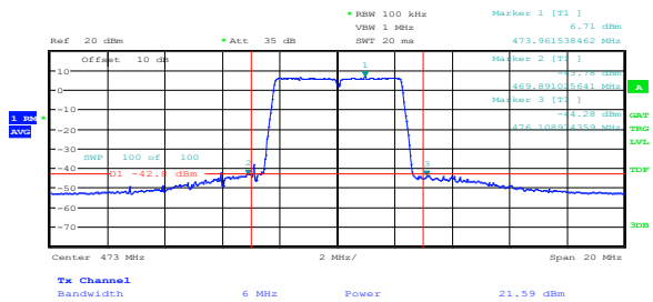
Figure 8.8-1: Conducted band edge and adjacent channel emissions sample plot for single 6 MHz channel
