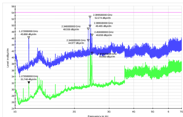
Figure 8.9-8: Radiated spurious emissions within 1–7 GHz for mid channel
