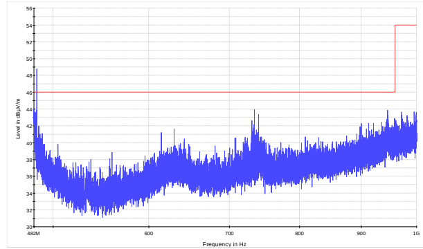
Figure 8.9-2: Radiated spurious emissions within 482–1000 MHz for low channel
