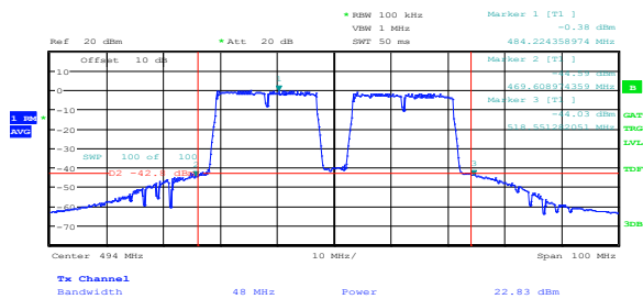
Figure 8.8-6: Conducted band edge and adjacent channel emissions sample plot for multi 24 MHz channel
