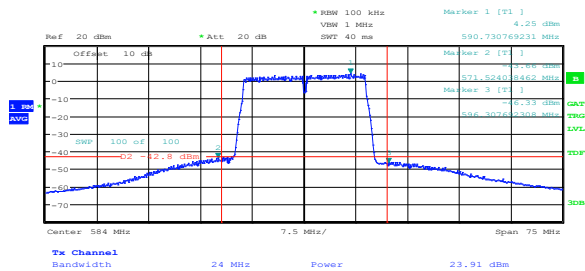
Figure 8.8-3: Conducted band edge and adjacent channel emissions sample plot for single 24 MHz channel
