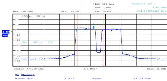
Figure 8.7-4: PSD within 100 kHz and Power within 6 MHz sample plot for multi 6 MHz channel
