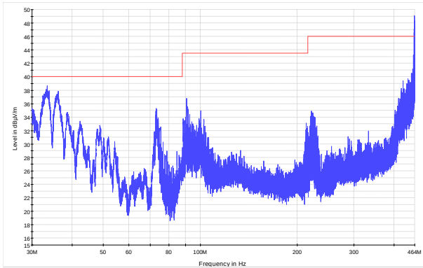
Figure 8.9-1: Radiated spurious emissions within 30–464 MHz for low channel
