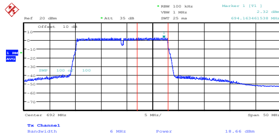
Figure 8.7-3: PSD within 100 kHz and Power within 6 MHz sample plot for single 24 MHz channel
