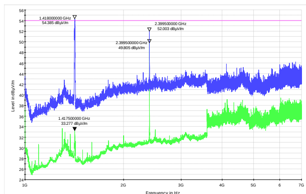
Figure 8.9-7: Radiated spurious emissions within 1–7 GHz for low channel
