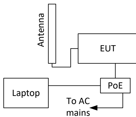
Figure 3.6-1: Setup diagram
