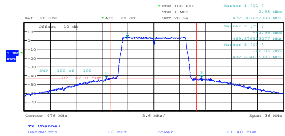
Figure 8.8-2: Conducted band edge and adjacent channel emissions sample plot for single 12 MHz channel
