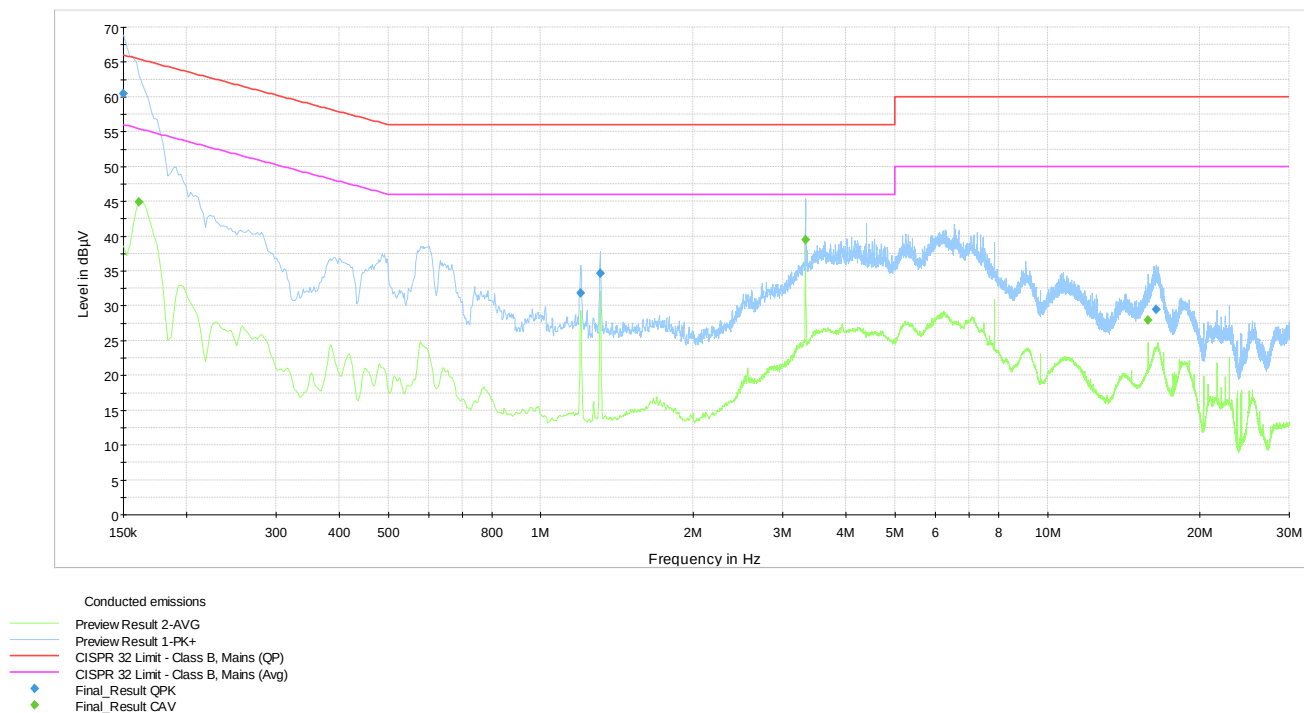
Plot 8.4-1: Conducted emissions on phase line
