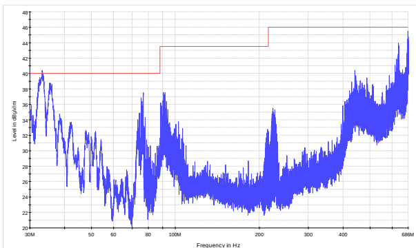
Figure 8.9-5: Radiated spurious emissions within 30–686 MHz for high channel
