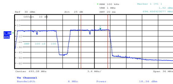
Figure 8.7-5: PSD within 100 kHz and Power within 6 MHz sample plot for multi 12 MHz channel
