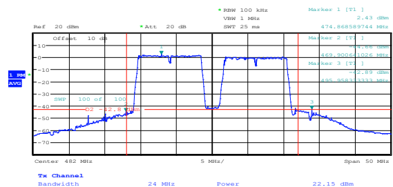
Figure 8.8-5: Conducted band edge and adjacent channel emissions sample plot for multi 12 MHz channel
