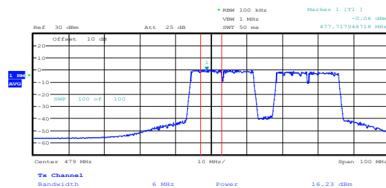
Figure 8.7-6: PSD within 100 kHz and Power within 6 MHz sample plot for multi 24 MHz channel
