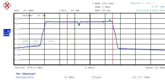
Figure 8.7-2: PSD within 100 kHz and Power within 6 MHz sample plot for single 12 MHz channel
