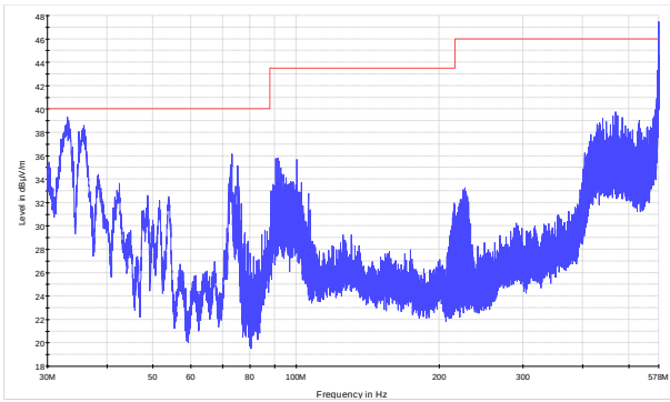
Figure 8.9-3: Radiated spurious emissions within 30–578 MHz for mid channel
