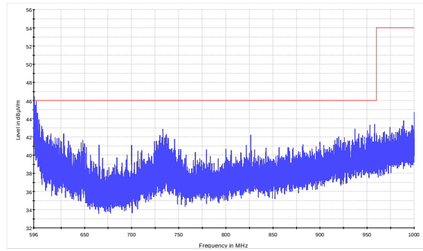
Figure 8.9-4: Radiated spurious emissions within 596–1000 MHz for mid channel
