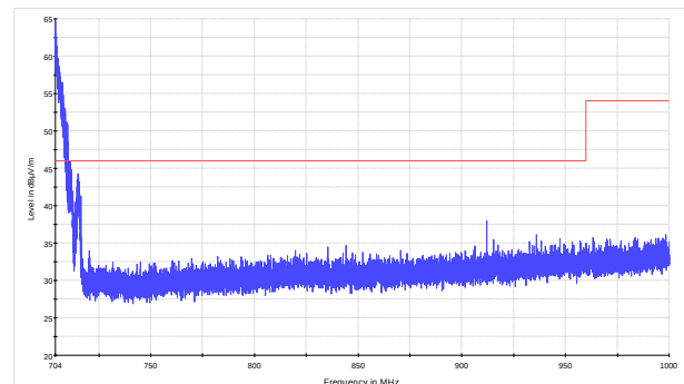
Figure 8.9-6: Radiated spurious emissions within 704–1000 MHz for high channel
