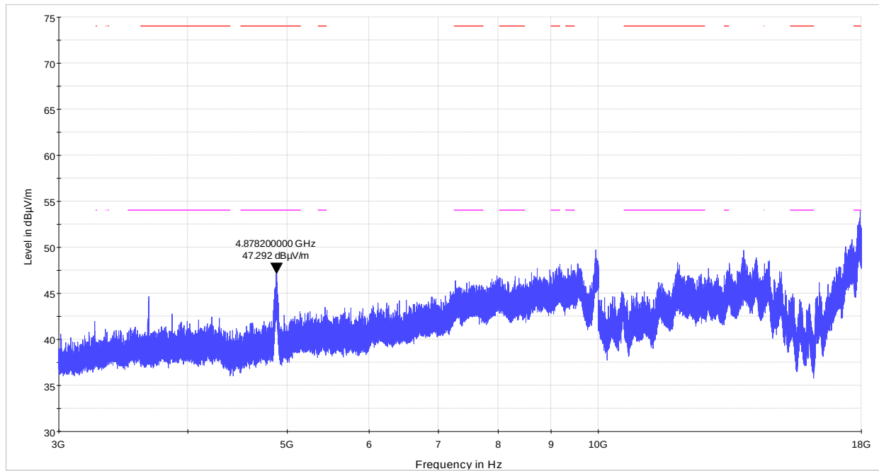
Figure 8.7-24: Radiated spurious emissions within 3–18 GHz for mid 40 MHz channel
