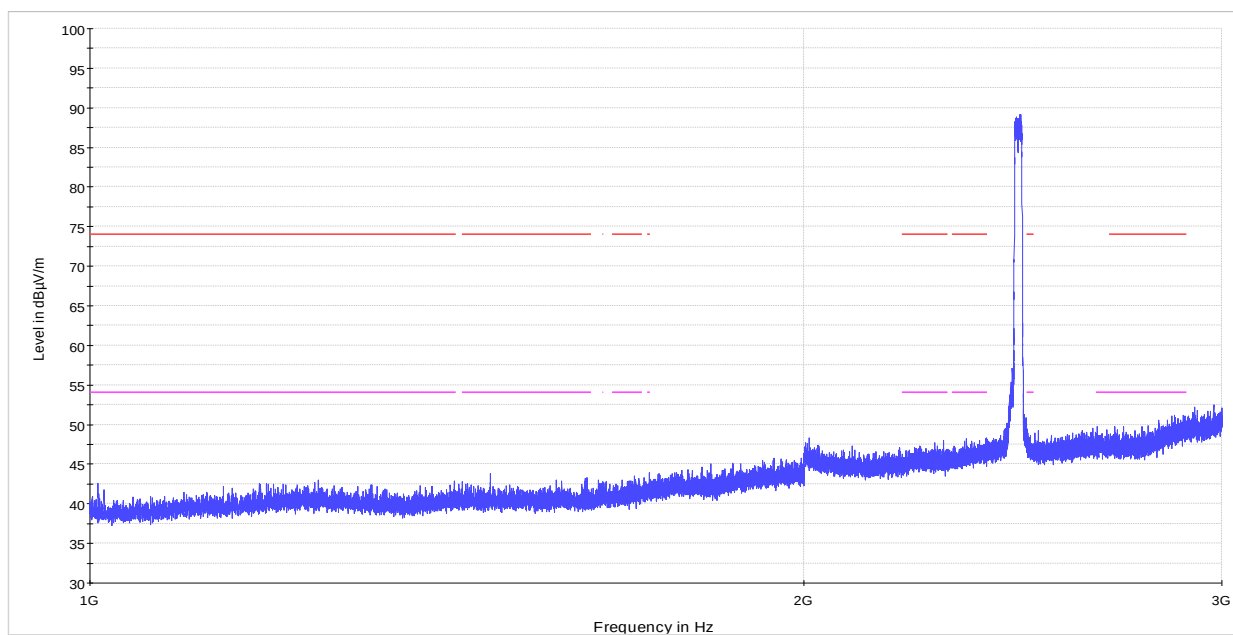
Figure 8.7-16: Radiated spurious emissions within 1–3 GHz for high 20 MHz channel
