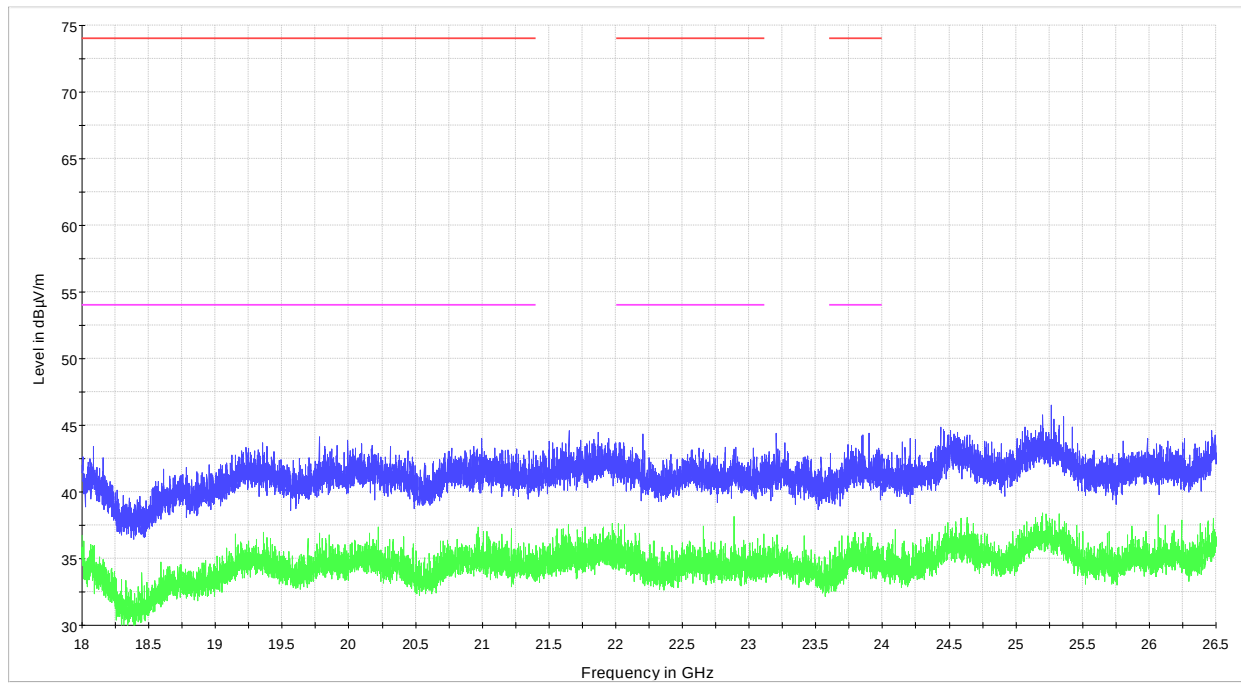
Figure 8.7-31: Radiated spurious emissions above 18 GHz for high 40 MHz channel
