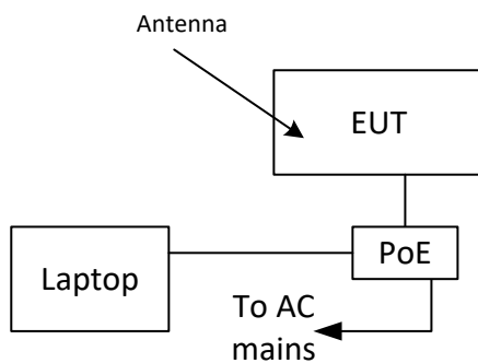
Figure 3.6-1: Setup diagram
