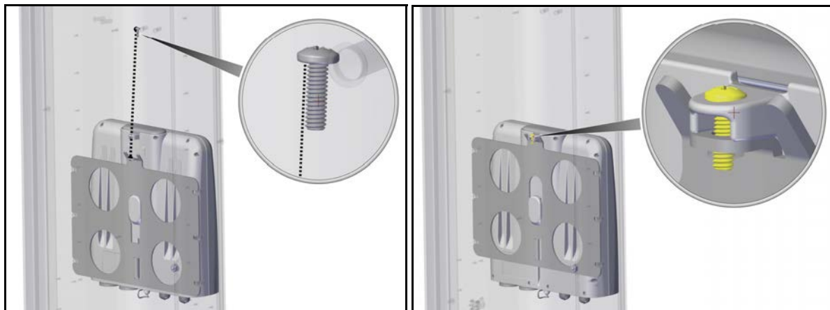
Figure 2-5: Fasten the locking screw
