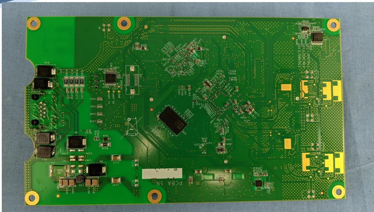
Main Board Bottom
