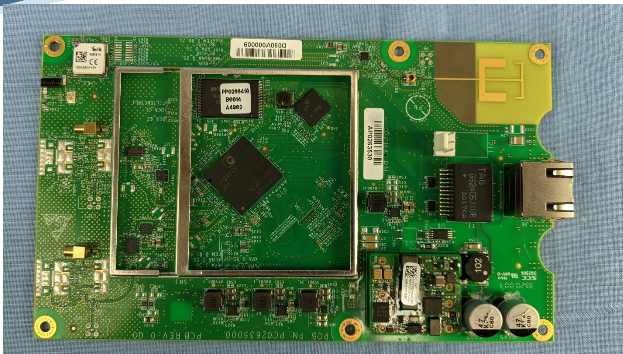
Main Board Top No Shield
