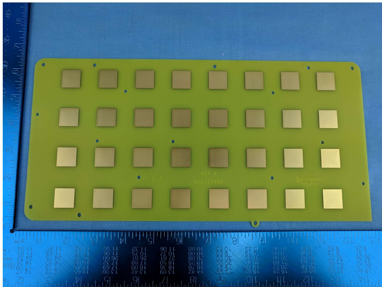
Antenna Assembly
