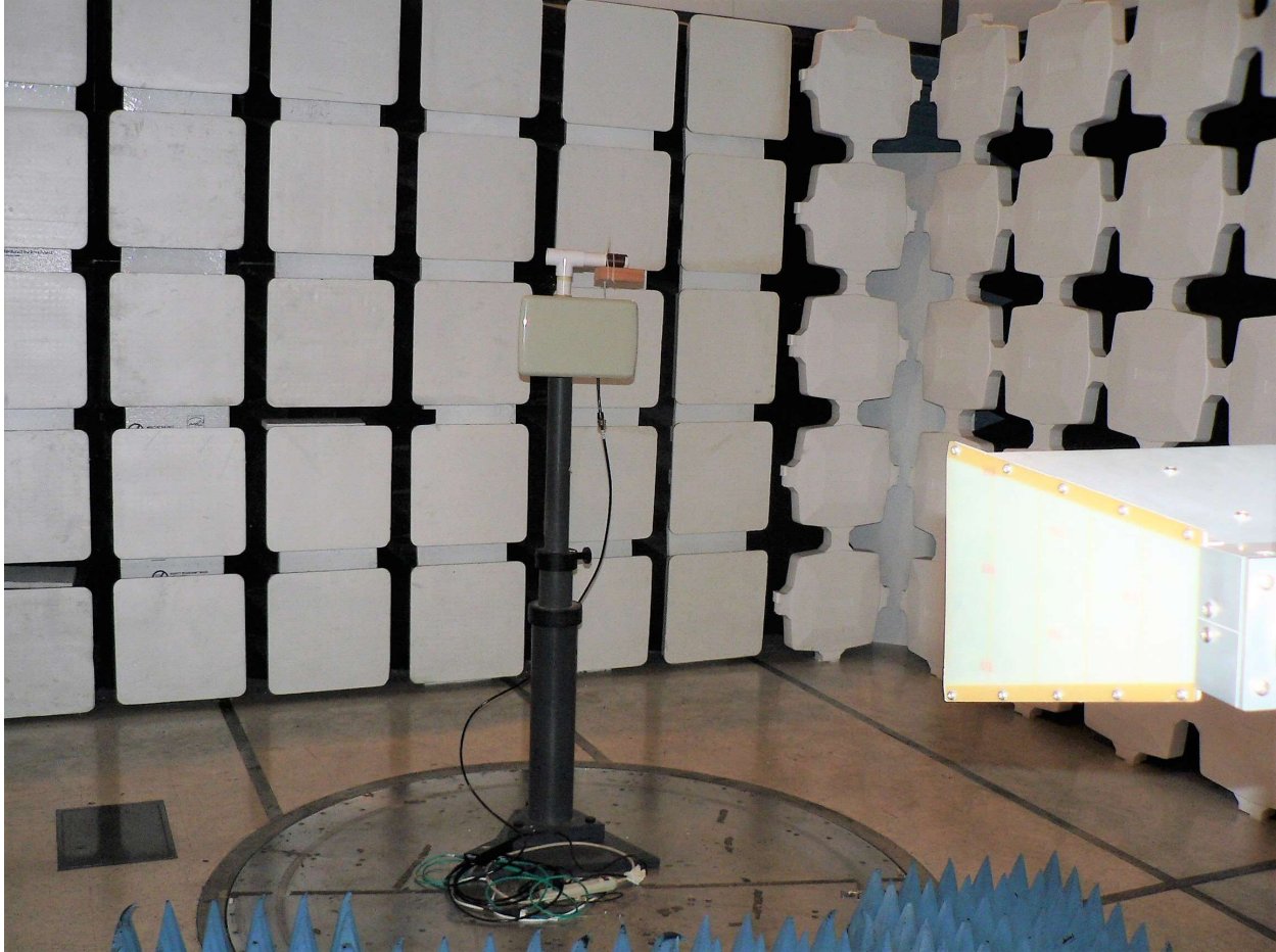
Radiated Emissions Antenna SA0183620
