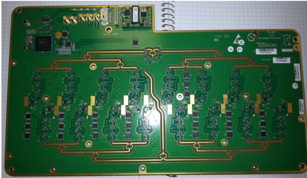
Photo #5: Smart Antenna PCB Rear
