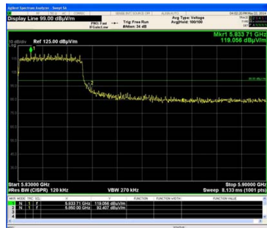
Plot # 115. Carrier frequency 5830 MHz.
