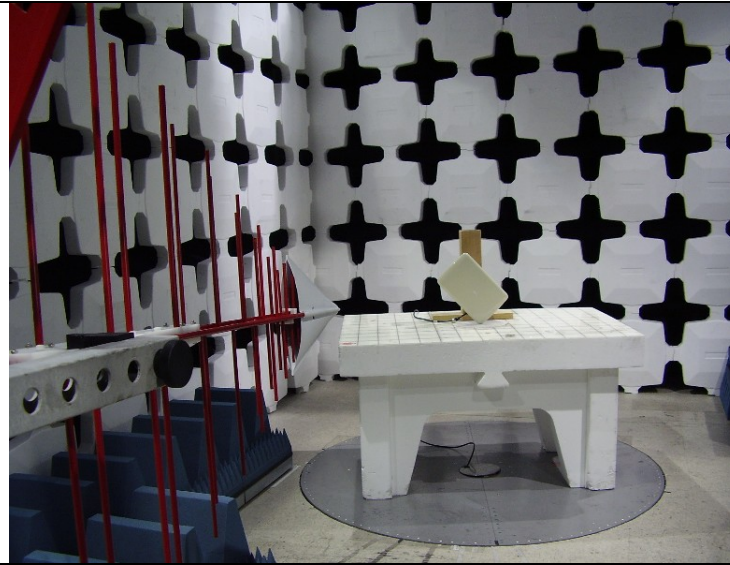
Photo #1. Radiated emission test setup.
