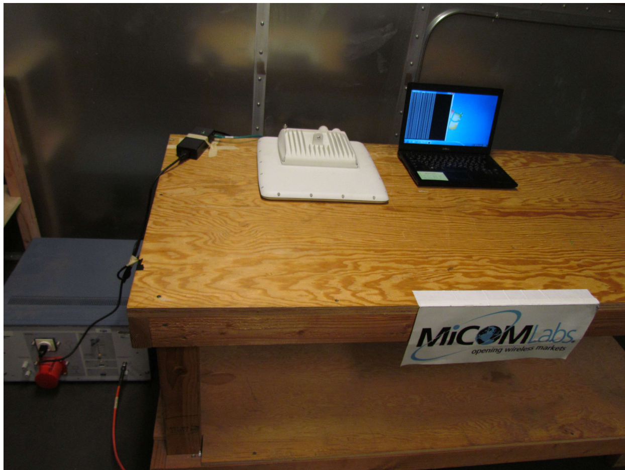
Conducted Emissions PoE configuration Front View
