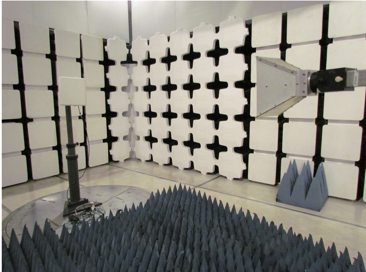
Radiated Emissions Antenna SA0199500
