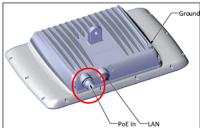
Figure 2-4: Laptop/network port: JET radio unit
