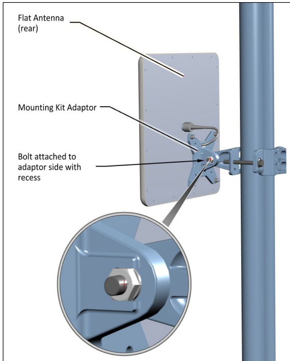
Figure 2-33: Flat Panel antenna - mounted on a pole
