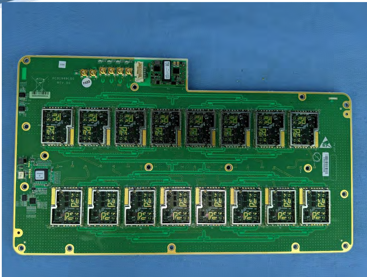
Upper Array Back Shields Removed
