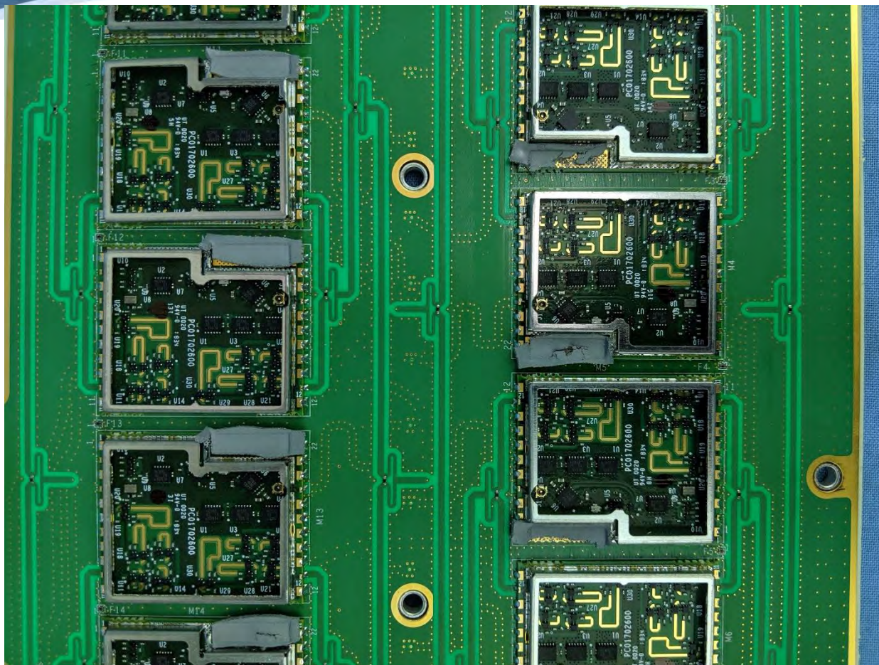
Lower Array RF Circuits 4-6 and 11-14
