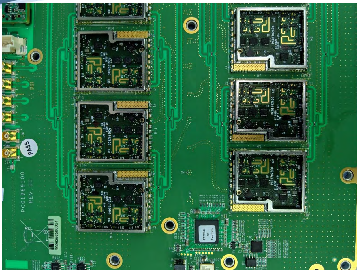
Upper Array RF Circuits 1-3 and 9-11
