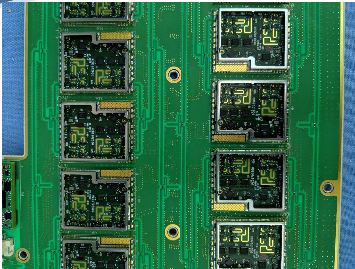
Upper Array RF Circuits 4-6 and 10-13
