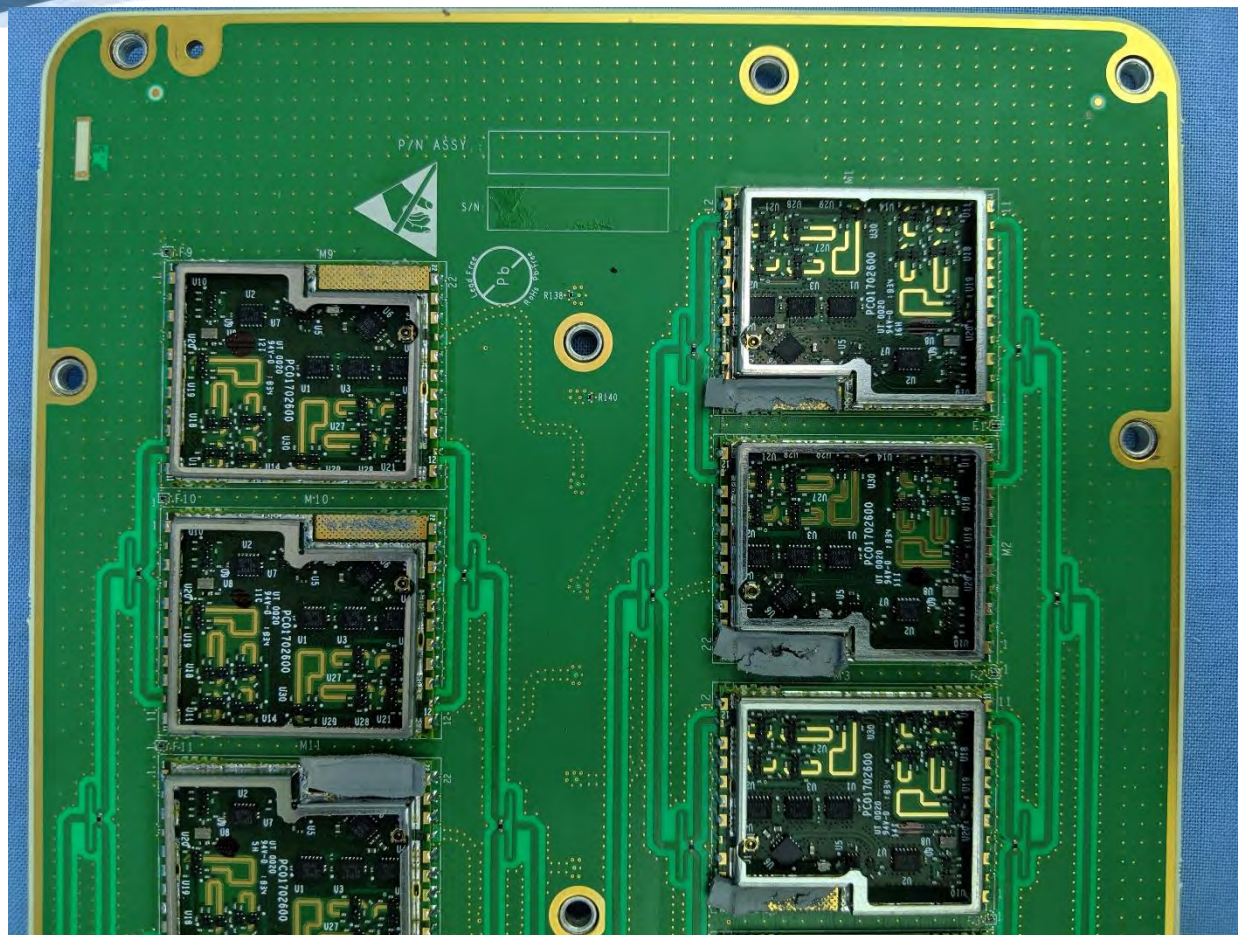
Lower Array RF Circuits 1-3 and 9-11
