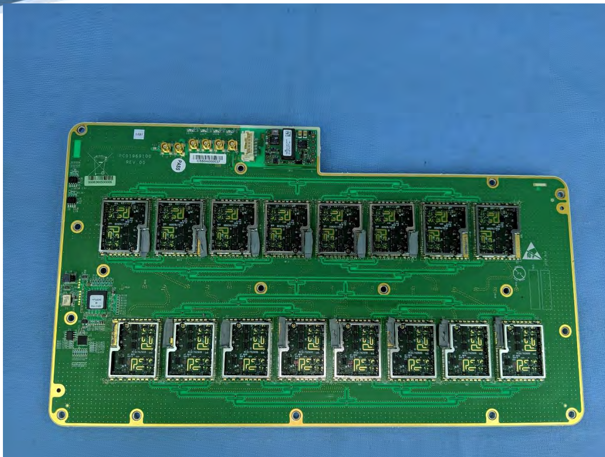
Lower Array Back Shields Removed
