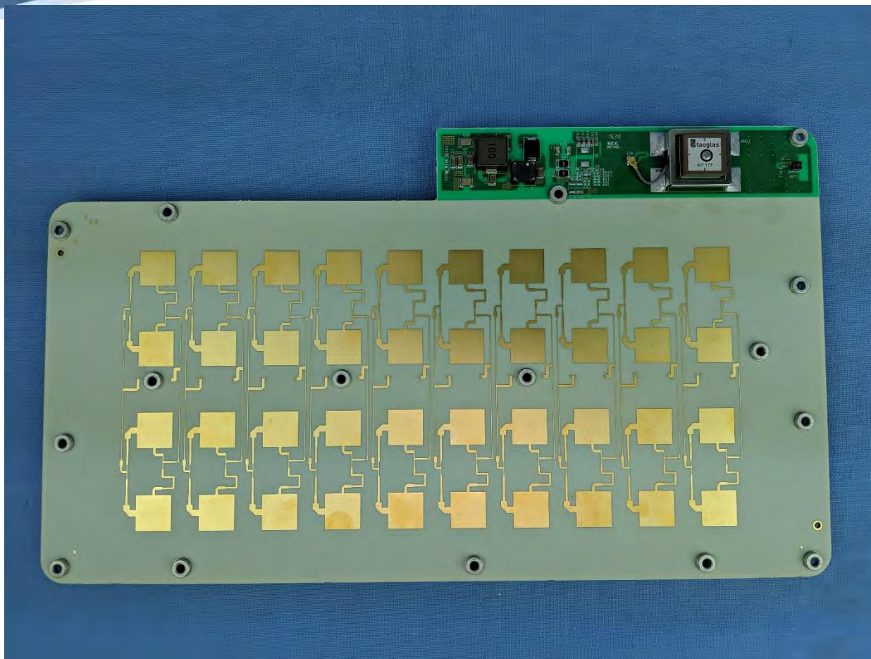
Upper Array Front
