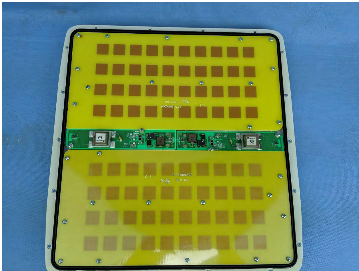
Full Antenna Array
