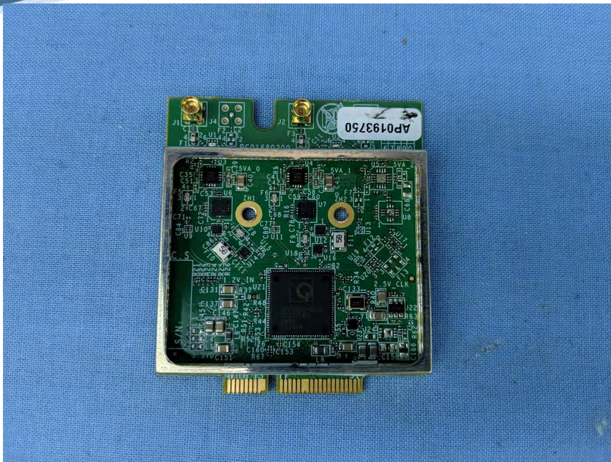
RF Module 1 Front
