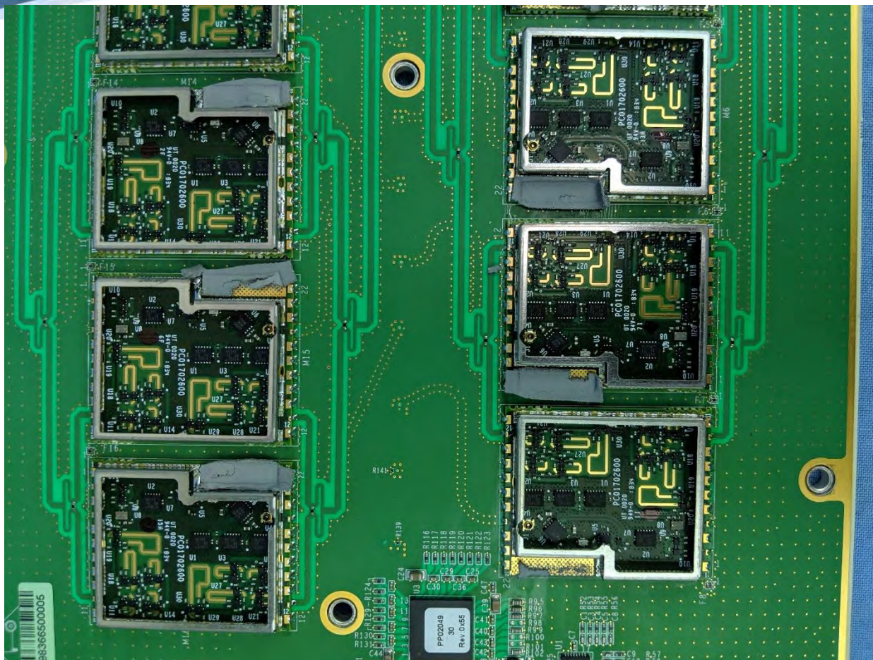
Lower Array RF Circuits 6-8 and 14-16
