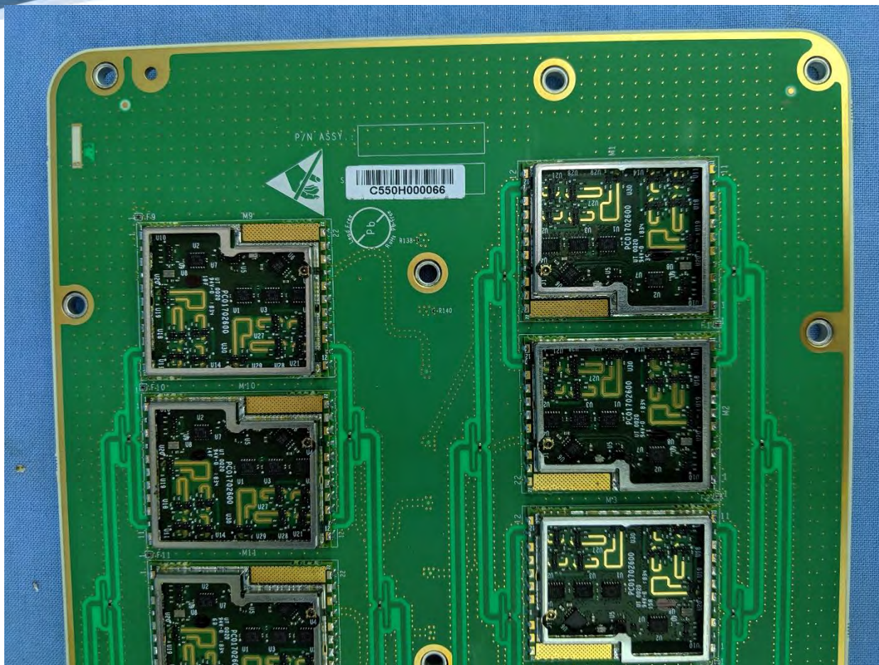
Upper Array RF Circuits 6-8 and 14-16
