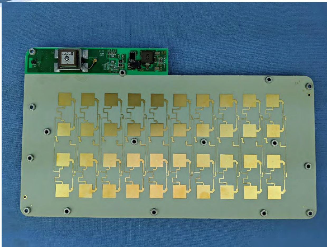
Lower Array Front
