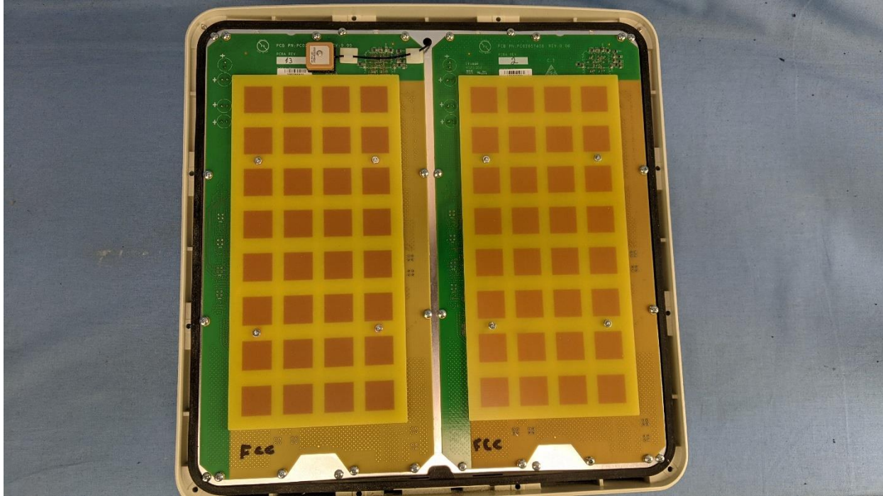
Antenna Assembly Front
