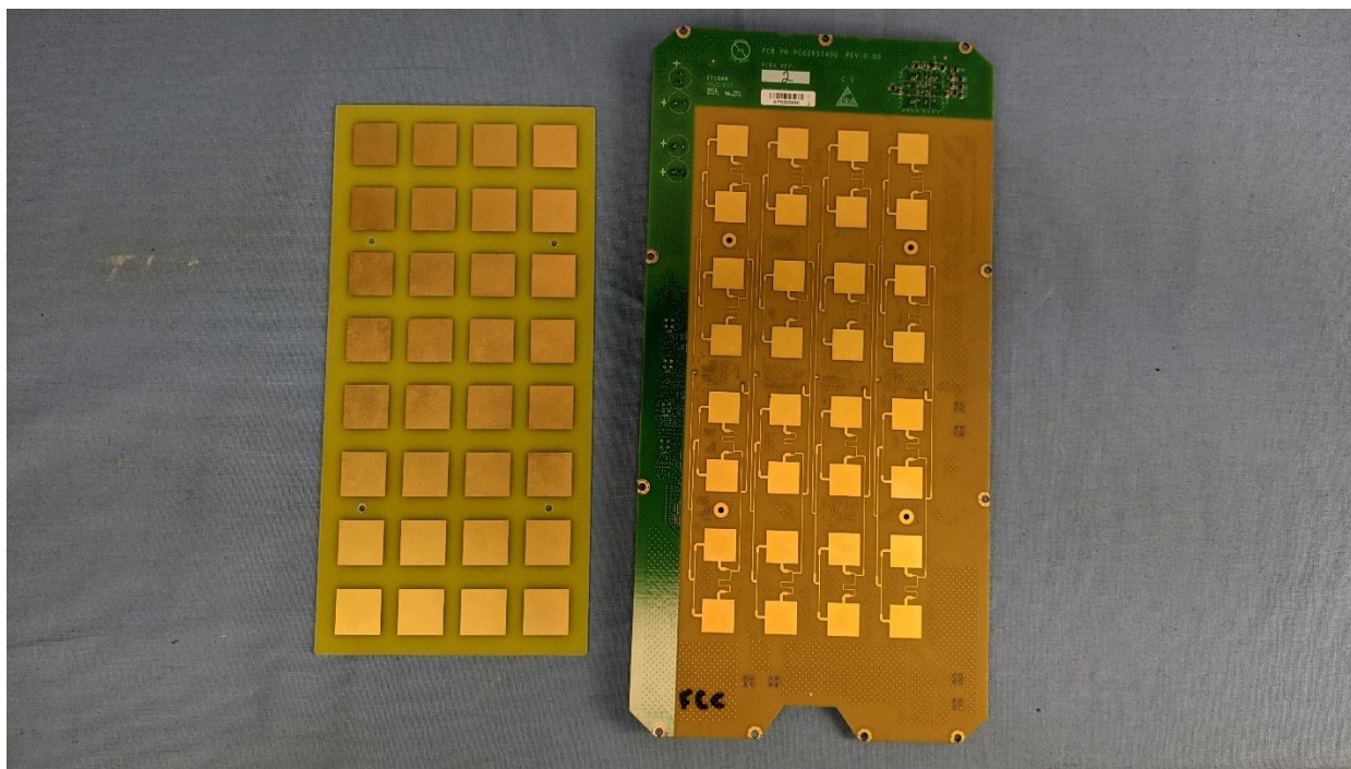
Right Antenna Assembly Front panel removed
