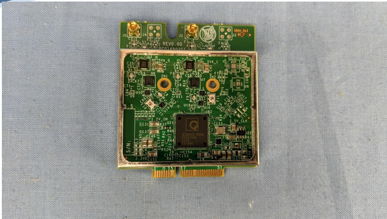
Right Radio Module Front Shield Removed
