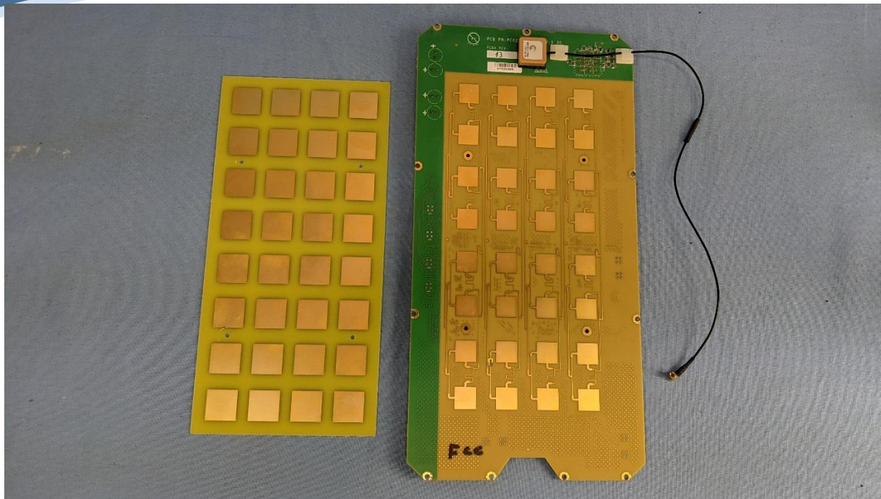
Left Antenna Assembly Front panel removed
