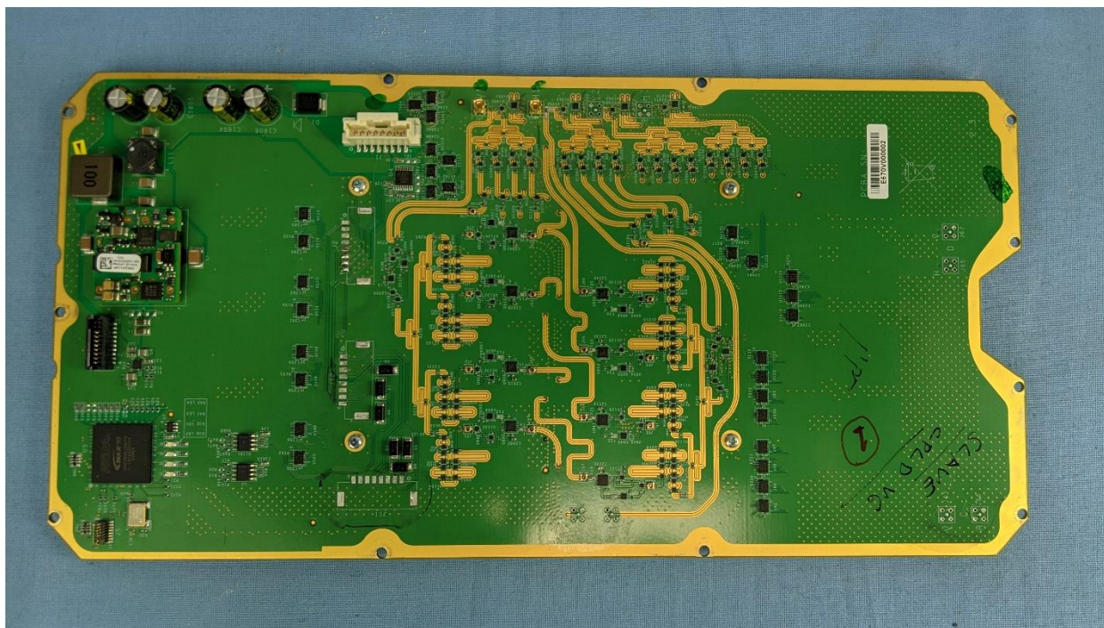
Right Antenna Assembly Back
