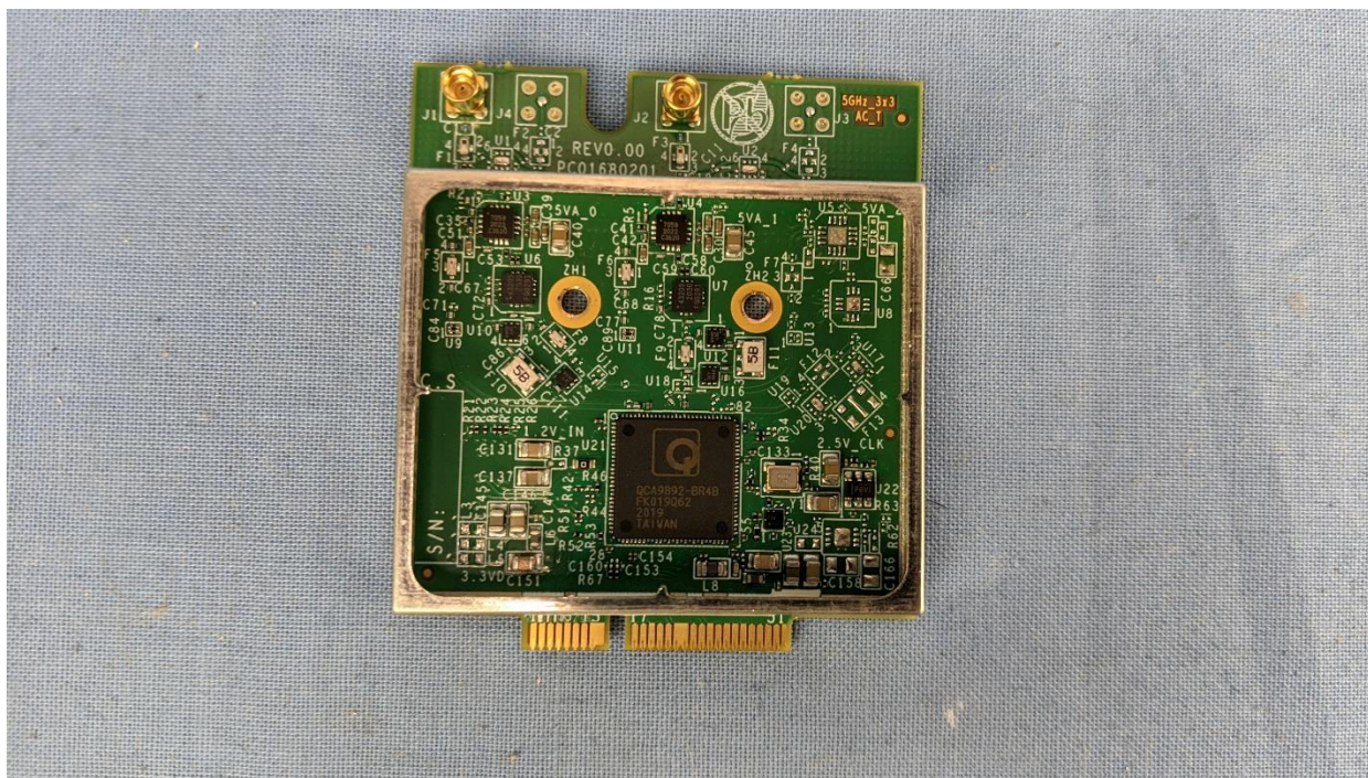
Left Radio Module Front Shield Removed
