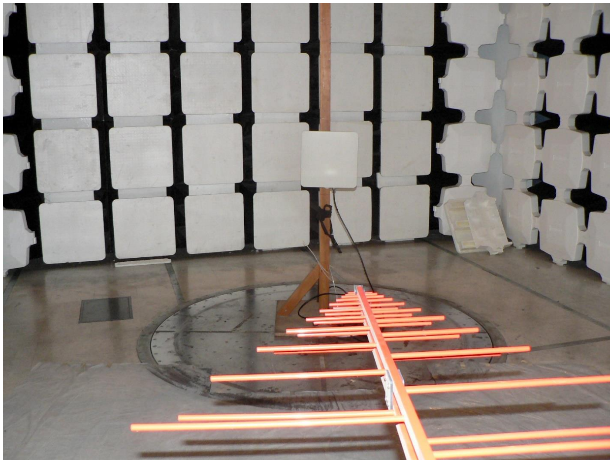
RDWN73 Digital Emissions 30-1000MHz
