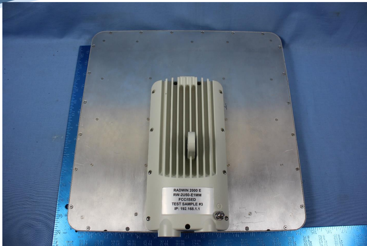
EUT with Integrated Antenna Back View
