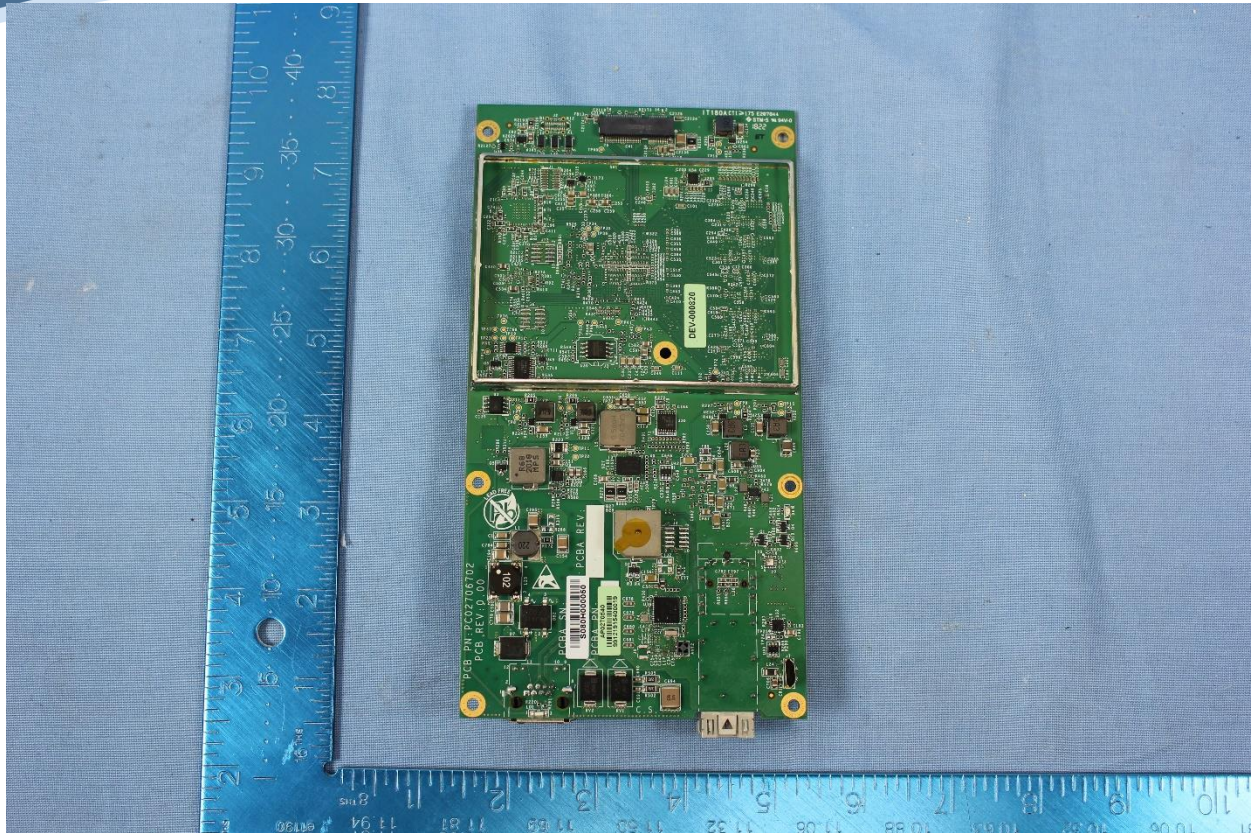
Main Board Front View
