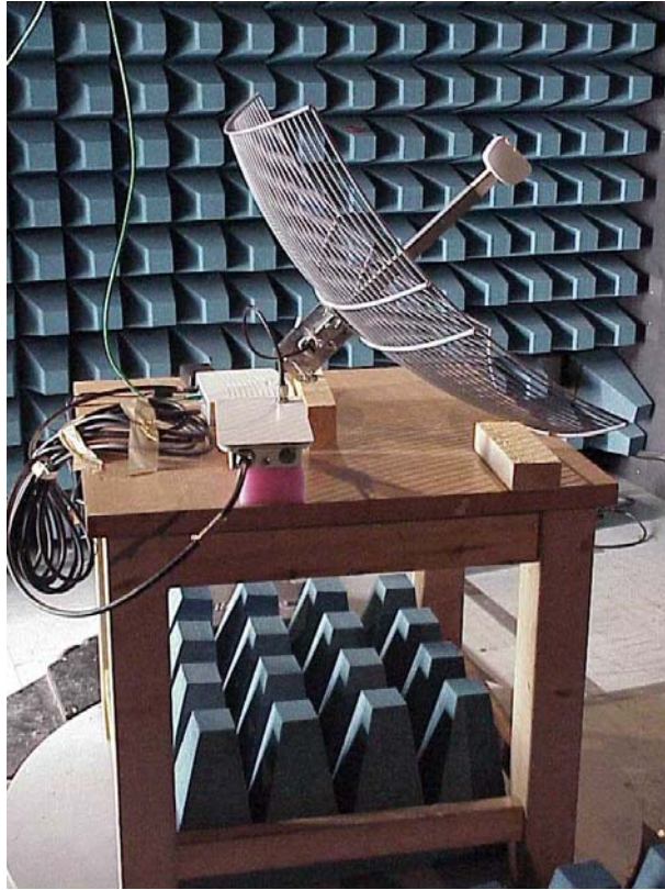
Spurious emissions measurements set up. External antenna
