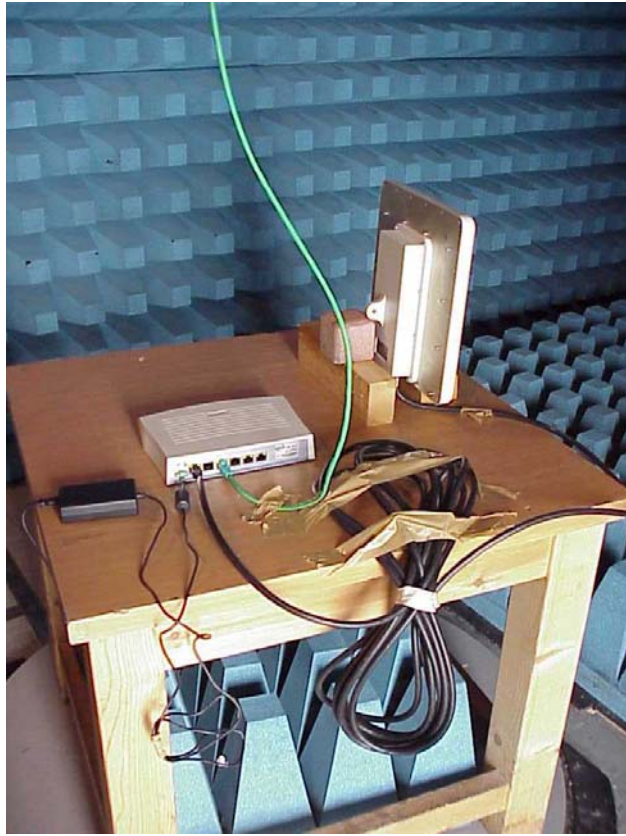
Spurious emissions measurements set up. Internal antenna
