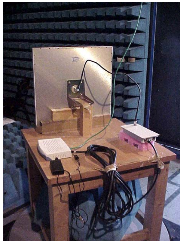
External antenna
