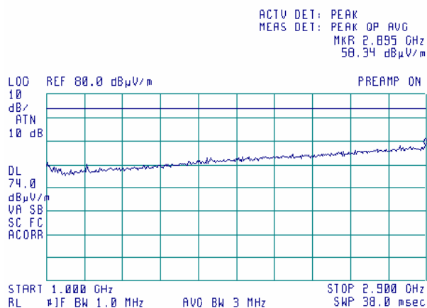
Plot 7.6.7 Radiated emission measurements from 1000 to 2900 MHz at the low carrier frequency
