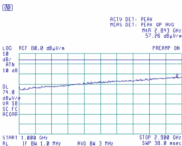
Plot 7.7.11 Radiated emission measurements from 1000 to 2900 MHz at the high carrier frequency
