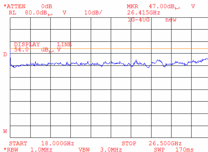
Plot 7.6.38 Radiated emission measurements from 18000 to 26500 MHz at the high carrier frequency
