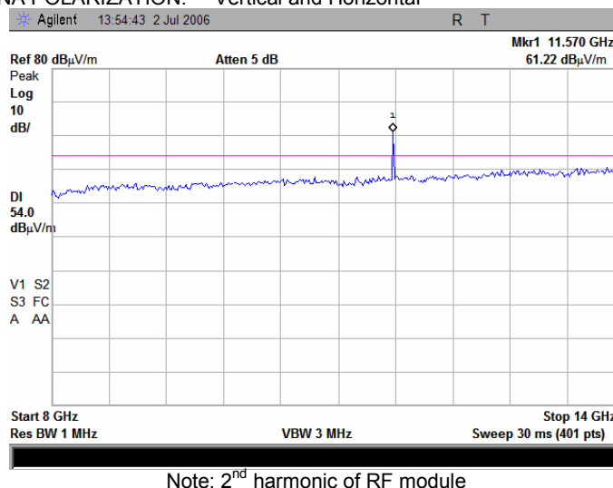
Plot 7.7.26 Radiated emission measurements from 8000 to 14000 MHz at the high carrier frequency
