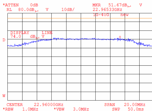
Plot 7.7.49 Radiated emission measurements at the forth harmonic of low carrier frequency
