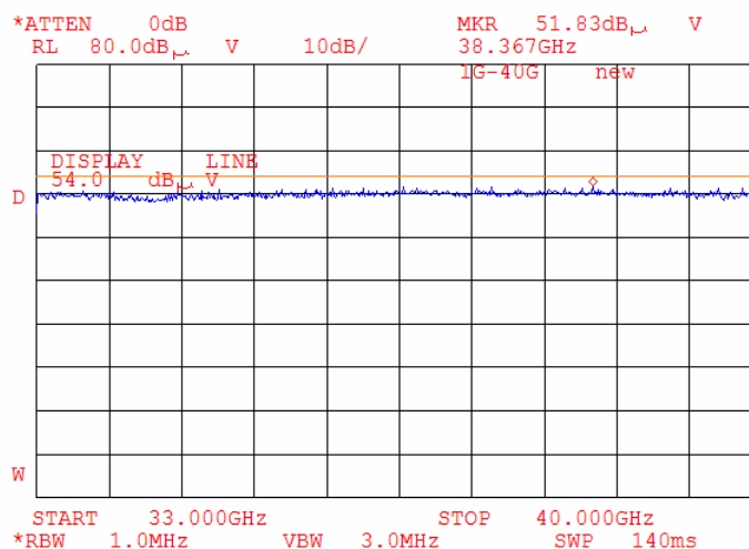
Plot 7.4.47 Radiated emission measurements from 33000 to 40000 MHz at the mid carrier frequency
