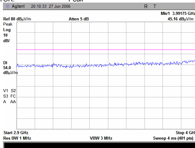
Plot 7.6.14 Radiated emission measurements from 2900 to 4000 MHz at the high carrier frequency
