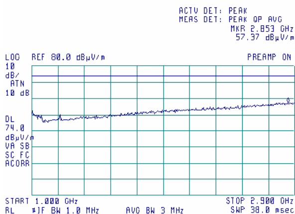
Plot 7.6.11 Radiated emission measurements from 1000 to 2900 MHz at the high carrier frequency
