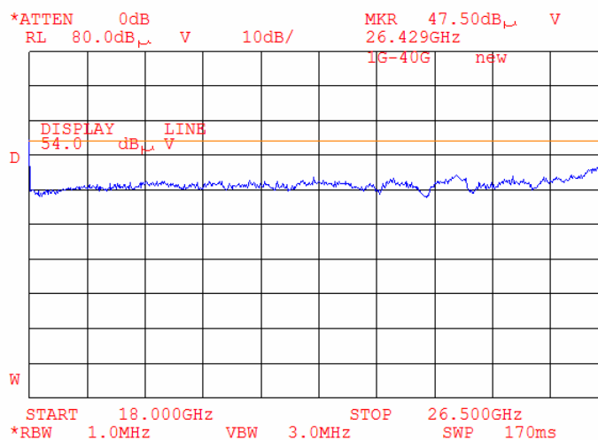
Plot 7.5.31 Radiated emission measurements from 18000 to 26500 MHz at the mid carrier frequency
