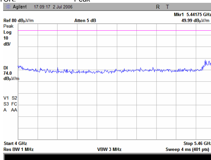
Plot 7.7.18 Radiated emission measurements from 4000 to 5460 MHz at the mid carrier frequency
