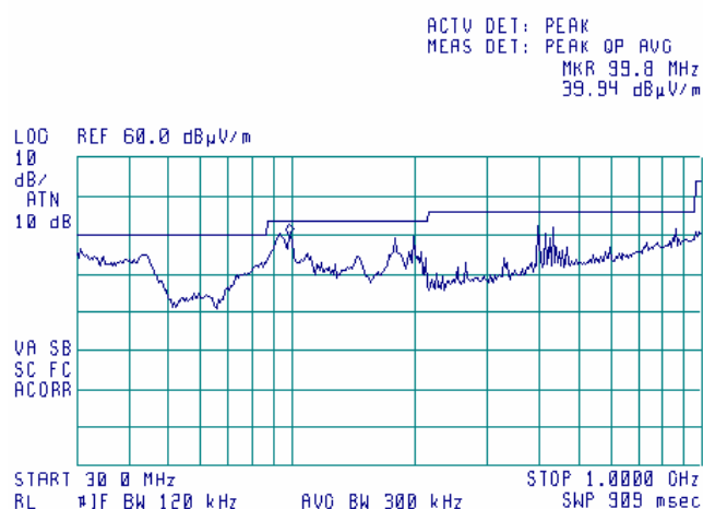
Plot 7.8.8 Radiated emission measurements from 30 to 1000 MHz at the mid carrier frequency
