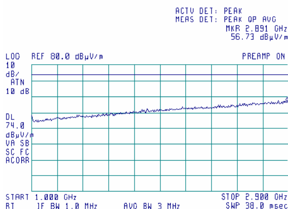
Plot 7.7.7 Radiated emission measurements from 1000 to 2900 MHz at the low carrier frequency
