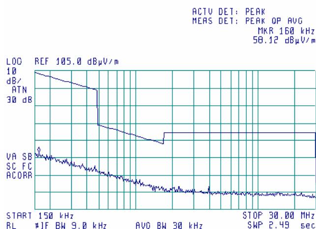
Plot 7.8.6 Radiated emission measurements from 0.15 to 30 MHz at the high carrier frequency
