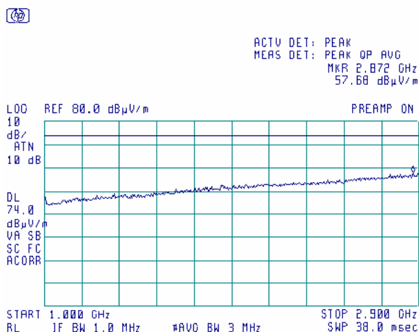
Plot 7.8.11 Radiated emission measurements from 1000 to 2900 MHz at the low carrier frequency
