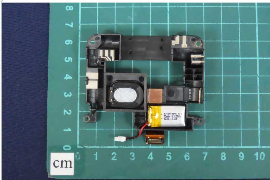
(26) EUT Photo
