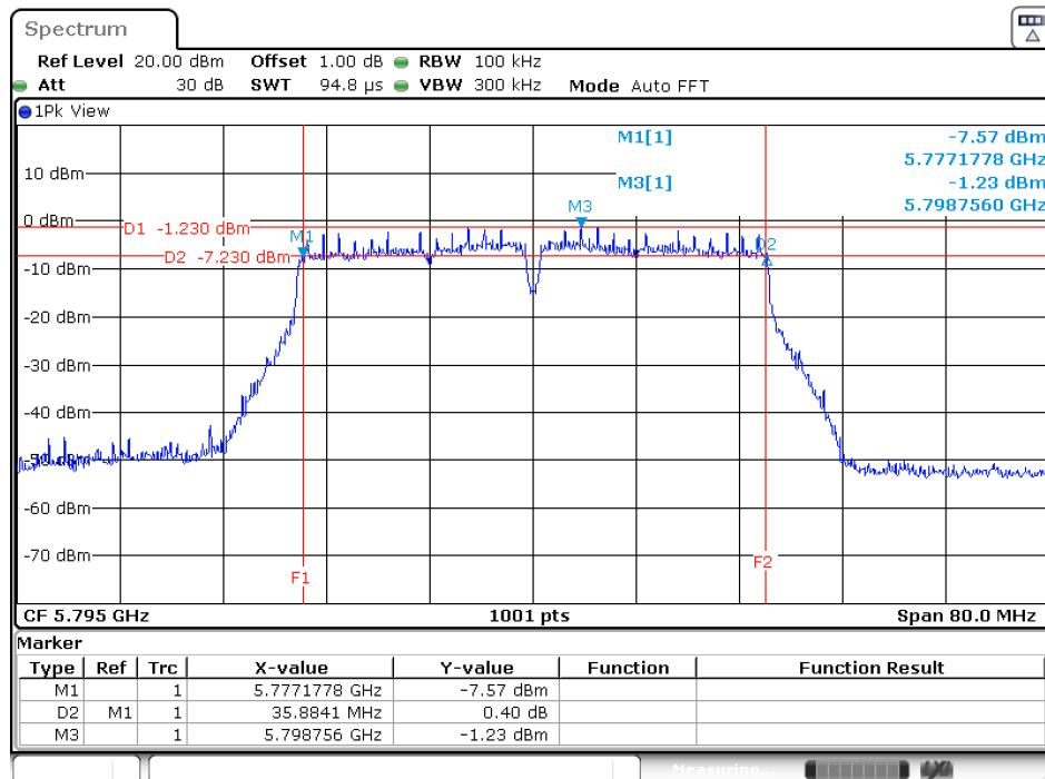
Channel 159
