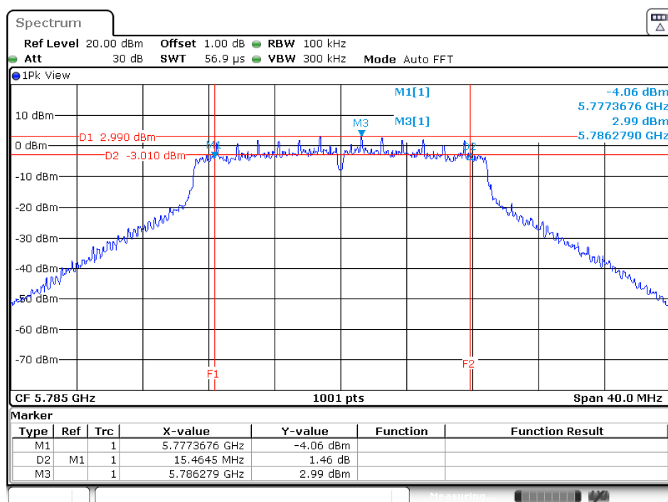
Channel 157
