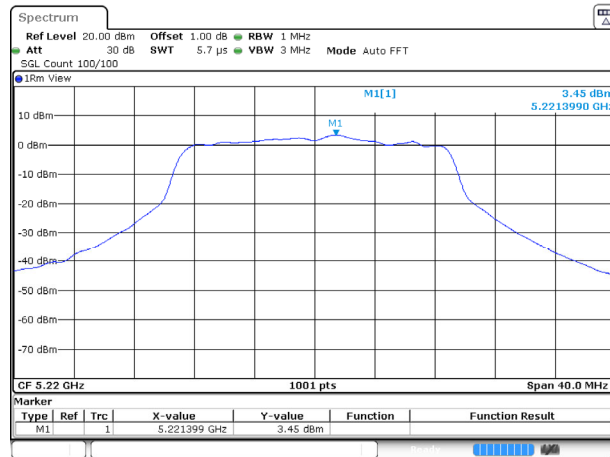
Channel 44
