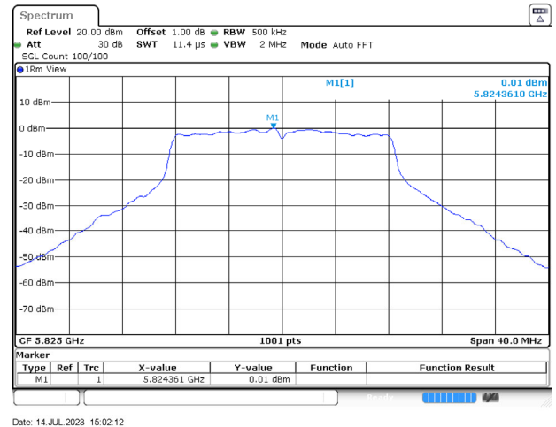
Channel 165
