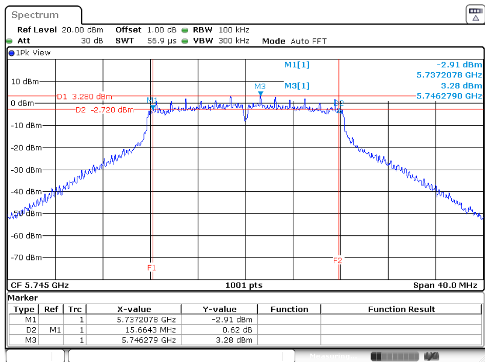
Channel 149
