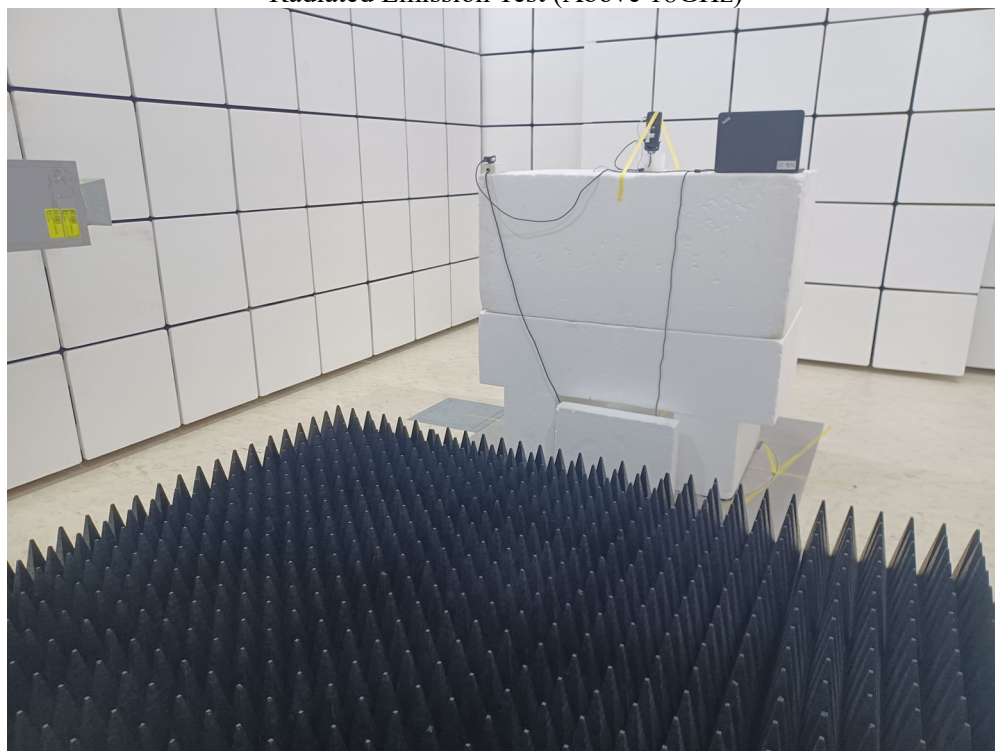
Radiated Emission Test (Above 18GHz)
