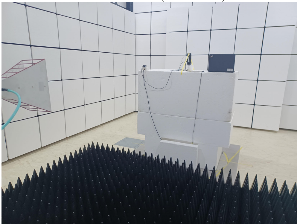
Radiated Emission Test (1GHz to 18GHz)
