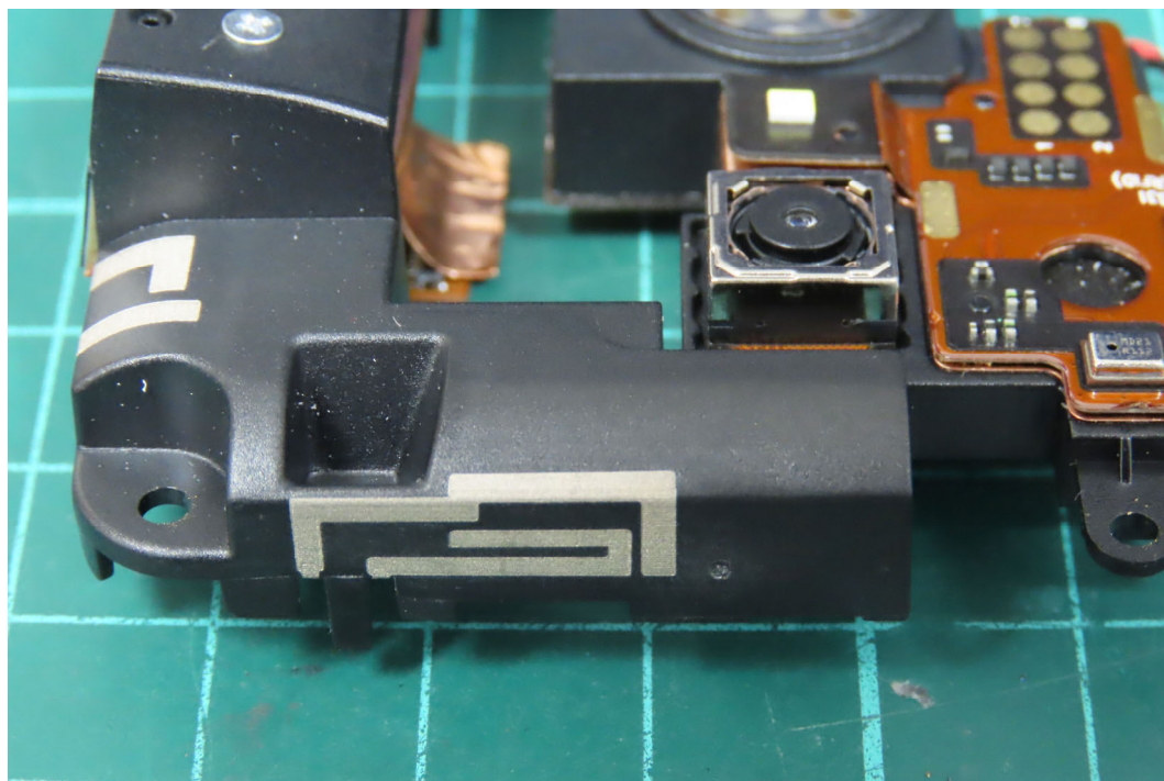
(22) EUT Photo
