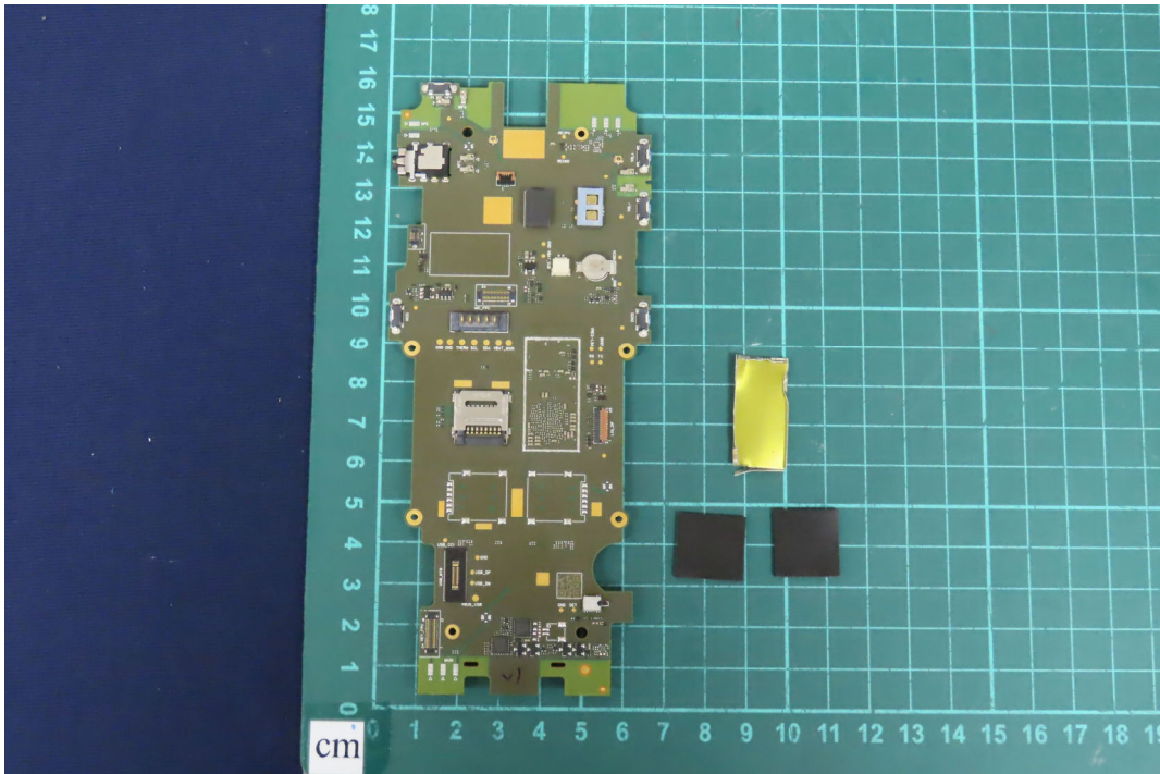
(32) EUT Photo
