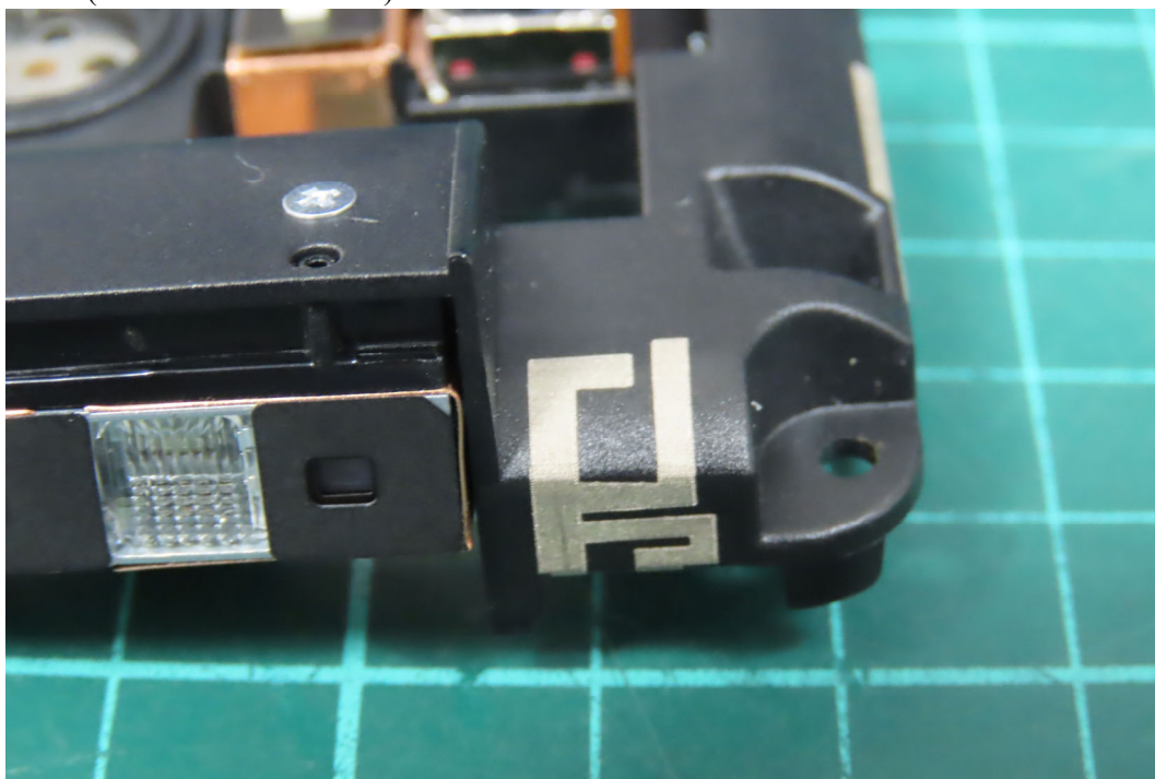
(23) EUT Photo (WLAN Main Antenna)
