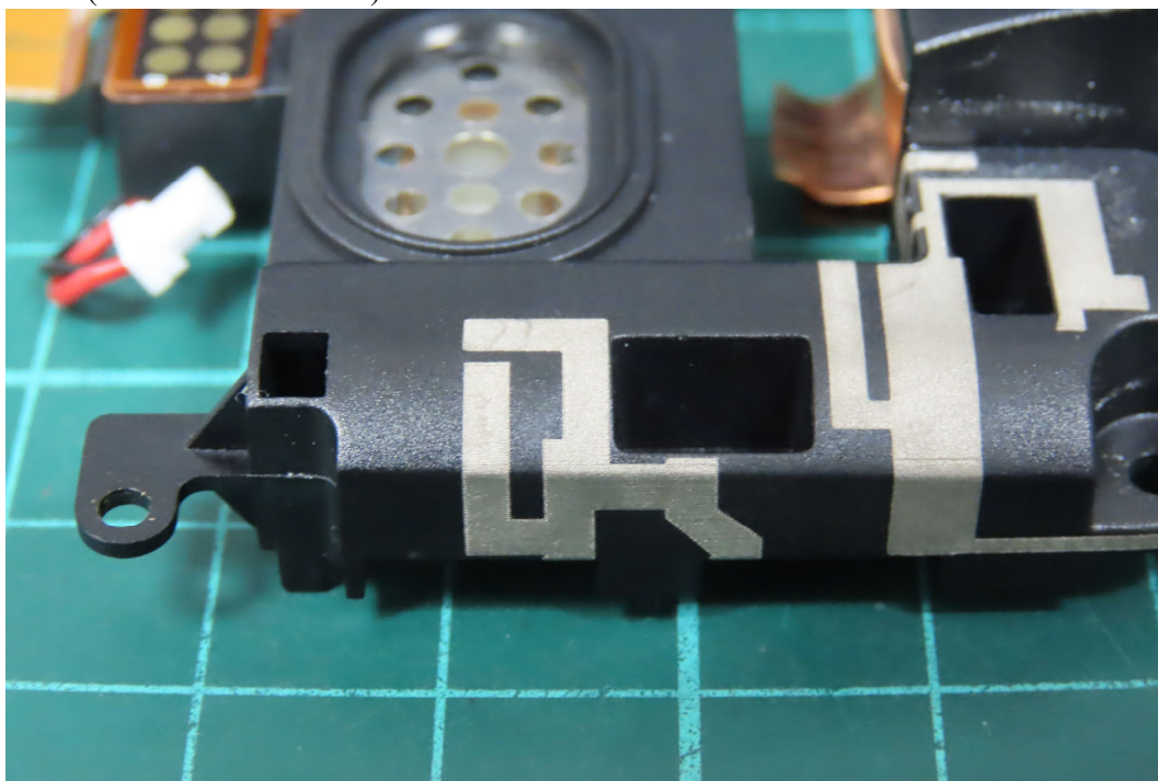
(25) EUT Photo (WLAN Aux Antenna)
