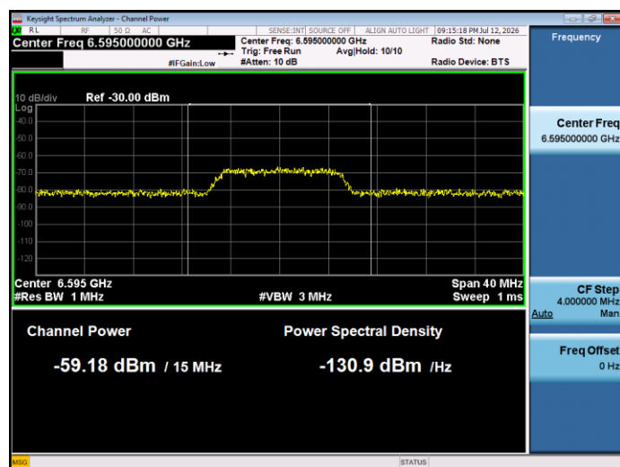
802.11ax (HE20)-Channel 129
