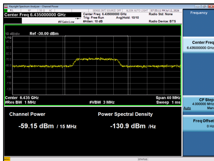
802.11ax (HE20)-Channel 97
