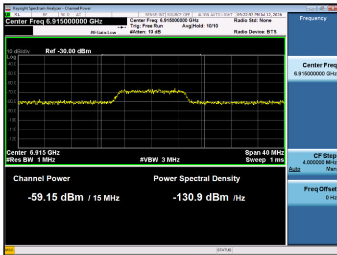
802.11ax (HE20)-Channel 193
