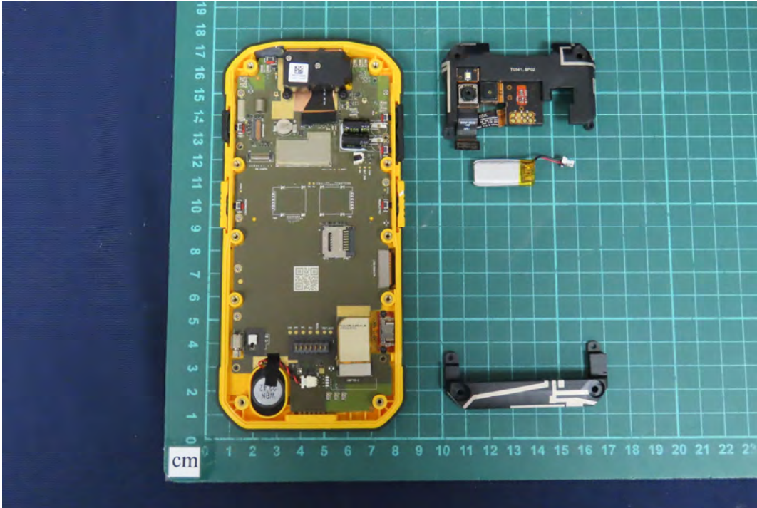
(7) EUT Photo
