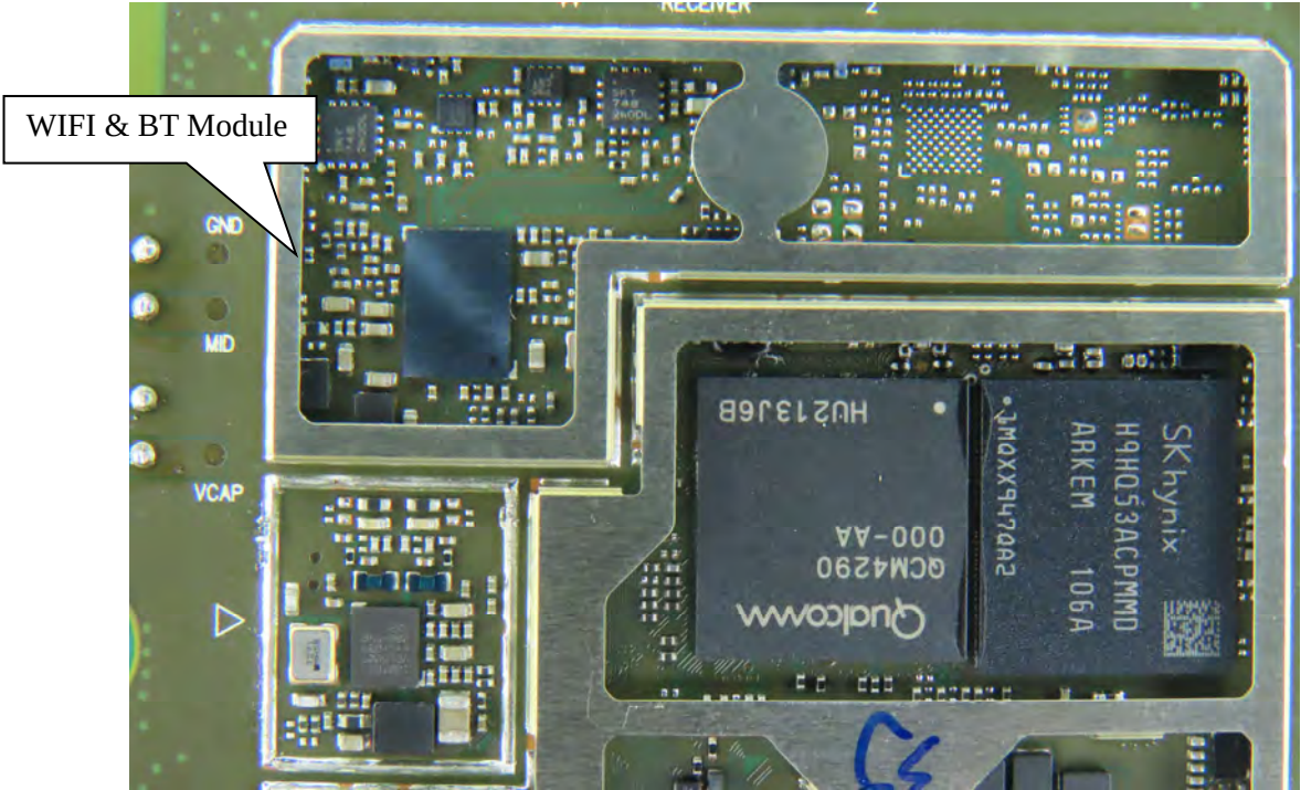
(25) EUT Photo
