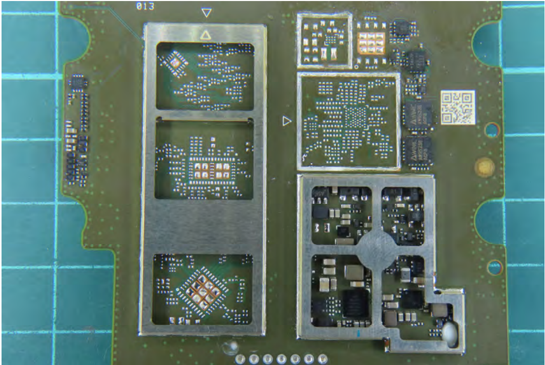
(29) EUT Photo
