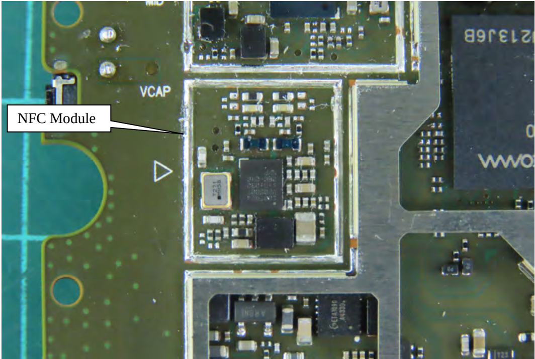
(27) EUT Photo
