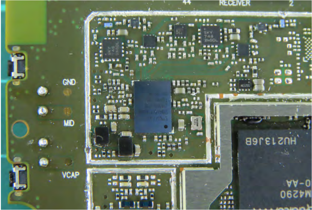
(26) EUT Photo
