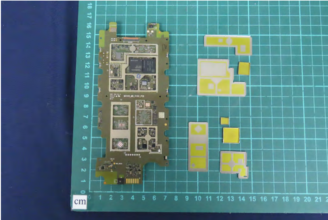
(23) EUT Photo
