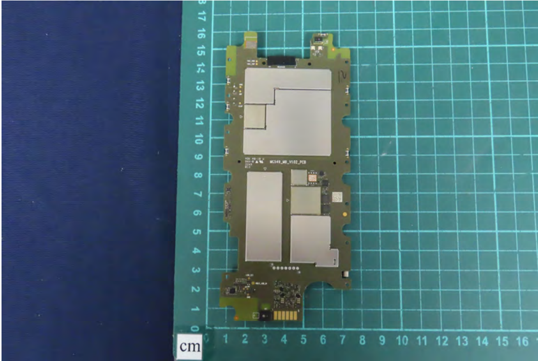
(22) EUT Photo
