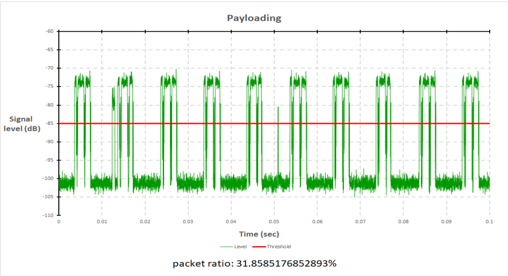
Plot of Slave Traffic at 5530 MHz
