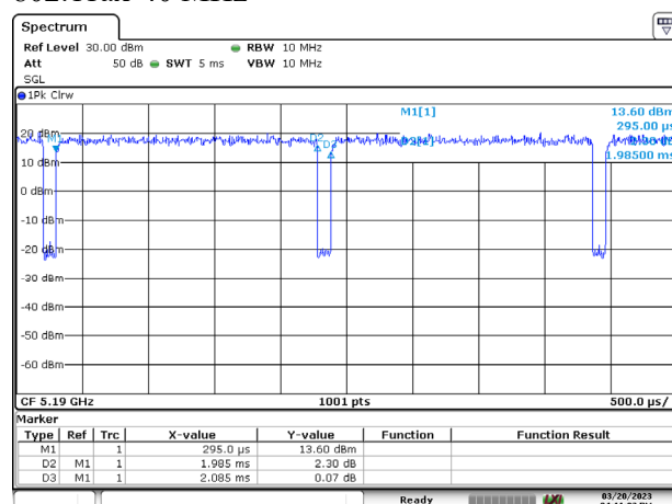
802.11ax-40 MHz
