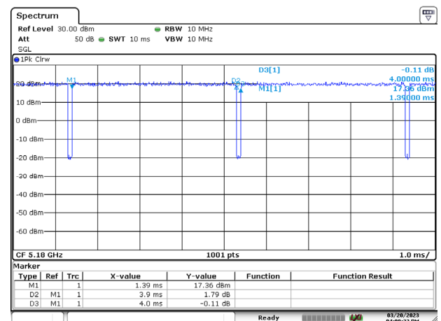
802.11ax-20 MHz
