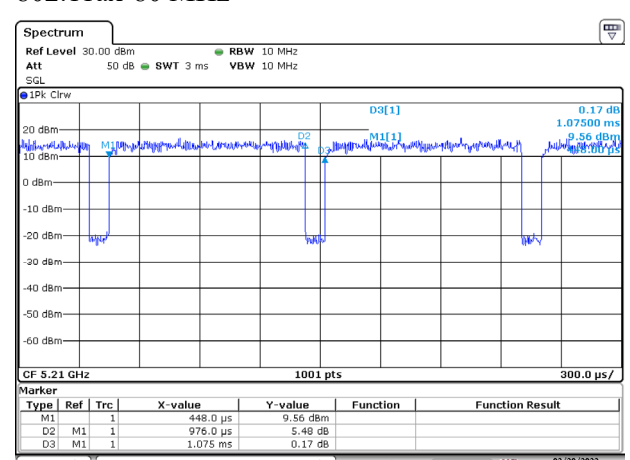
802.11ax-80 MHz
