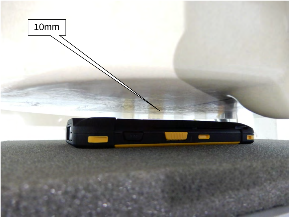
EUT Back_10mm
