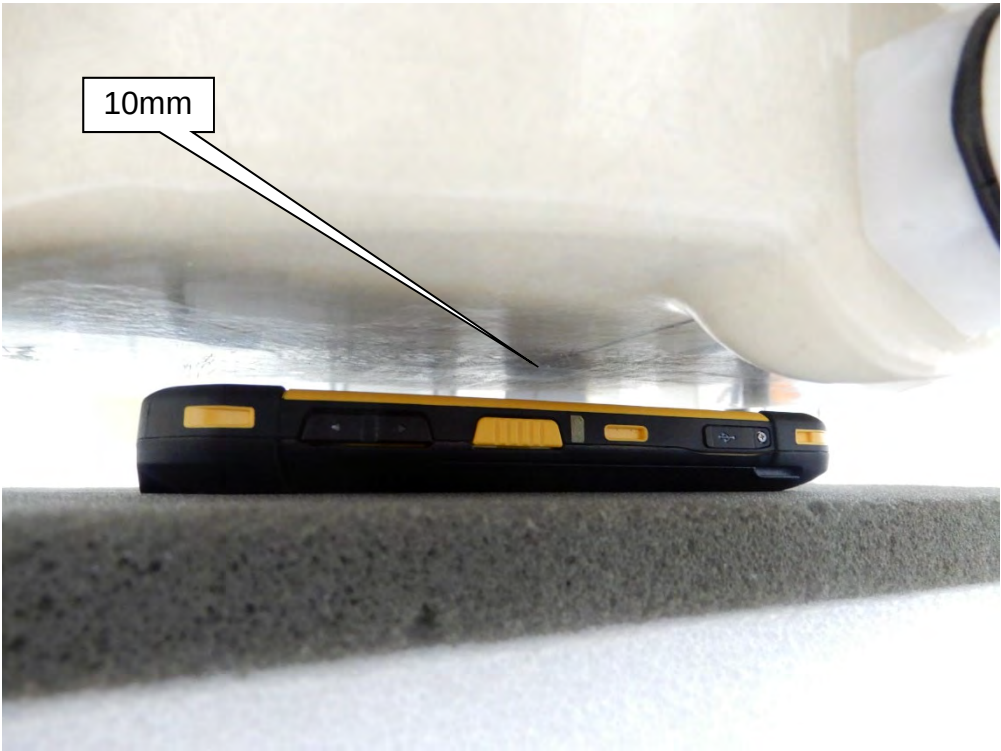
EUT Front_10mm
