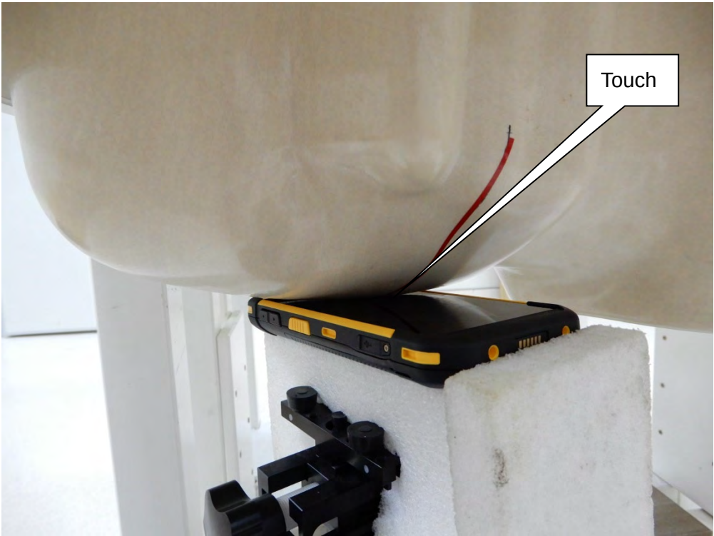
EUT Right-Cheek
