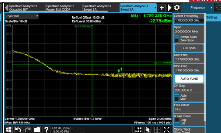
FULL CH 132374 (1750.2MHz) + 132572 (1770.0MHz)
