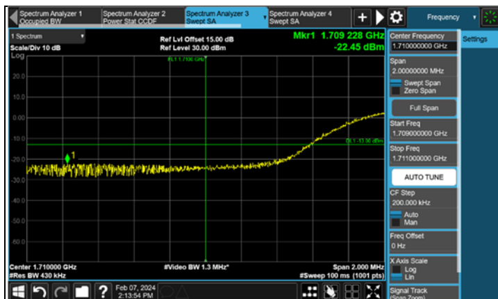
FULL CH 132072 (1720.0MHz) + 132270 (1739.8MHz)
