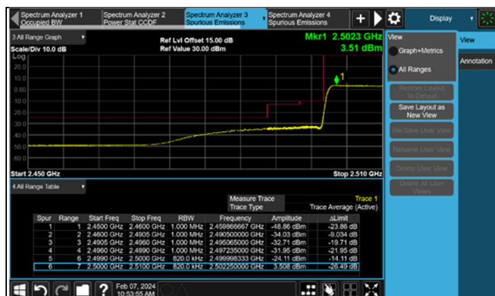
FULL CH 20850 (2510.0MHz) + 21048 (2529.8MHz)
