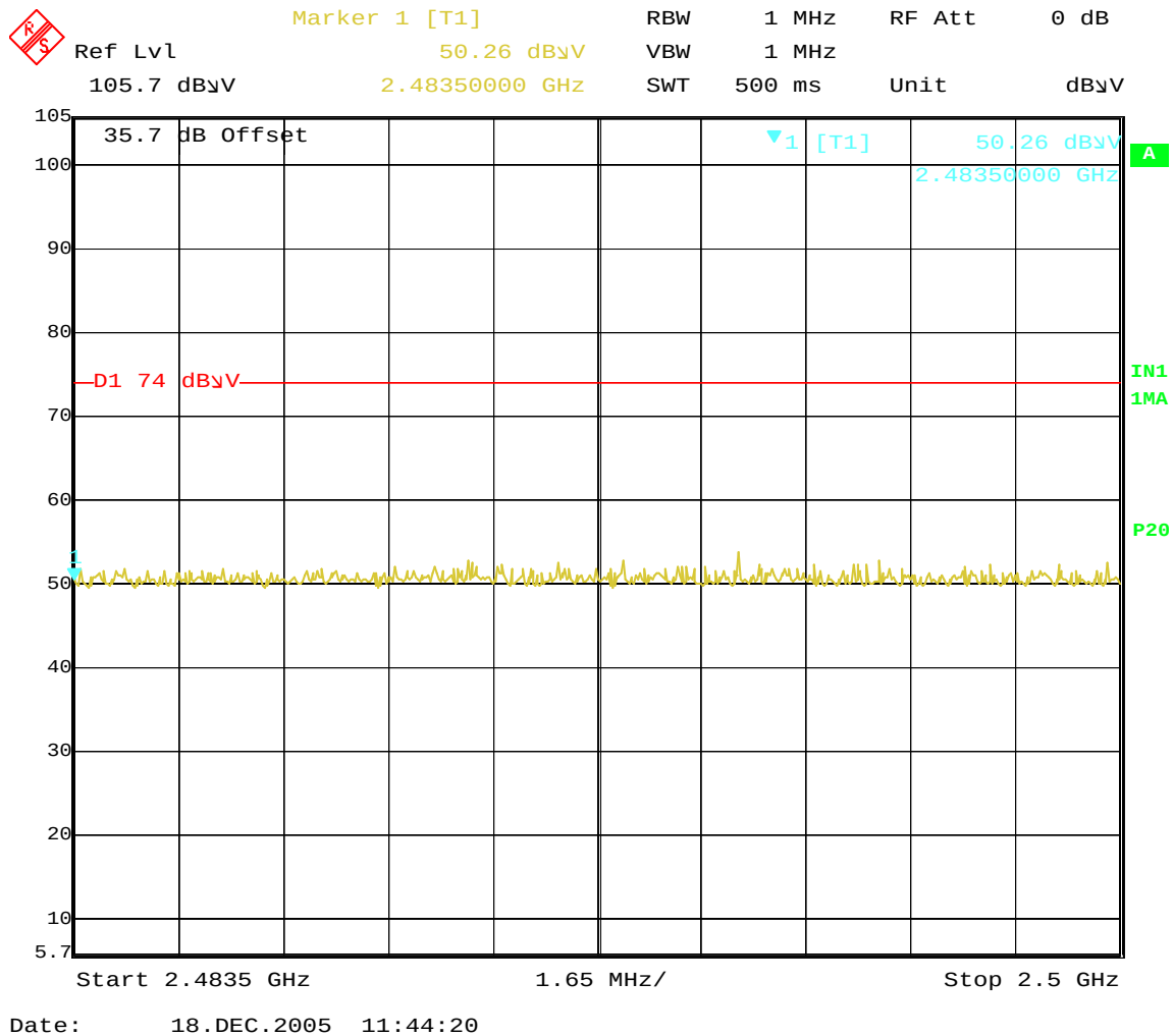
Figure 7-7: High Ch. Restricted Band; 802.11b Mode; Vertical Polarity; Peak Detection
