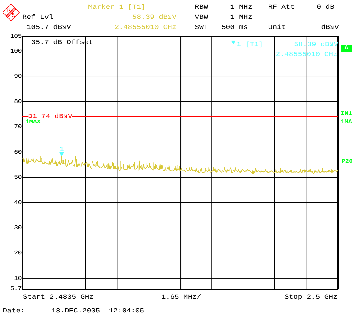
Figure 7-15: High Ch. Restricted Band; 802.11g Mode; Vertical Polarity; Peak Detection
