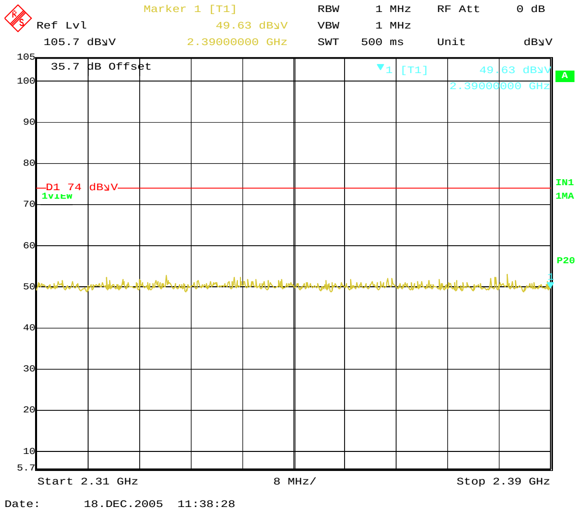
Figure 7-3: Low Ch. Restricted Band; 802.11b Mode; Vertical Polarity; Peak Detection
