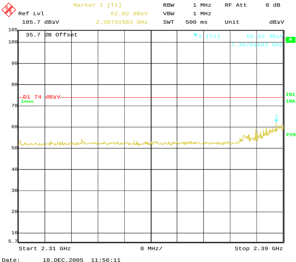
Figure 7-11: Low Ch. Restricted Band; 802.11g Mode; Vertical Polarity; Peak Detection
