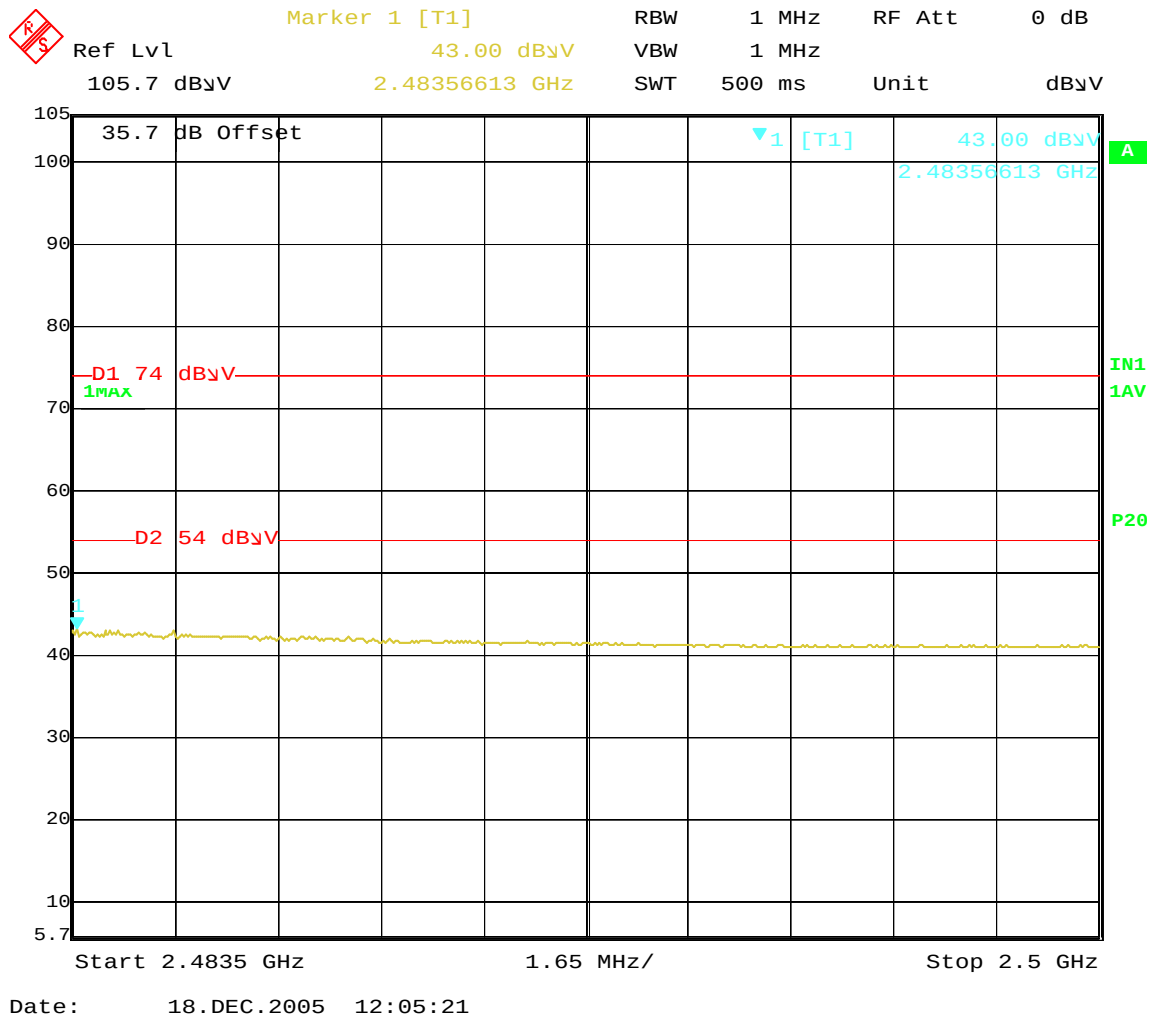
Figure 7-16: High Ch. Restricted Band; 802.11g Mode; Vertical Polarity; Avg. Detection
