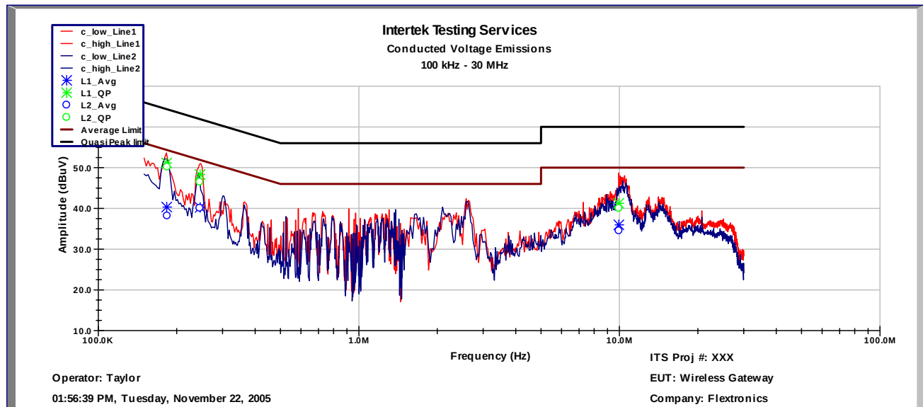
Figure 8-1: FCC §15. Power Line Conducted Emissions (Lines 1 and 2)
