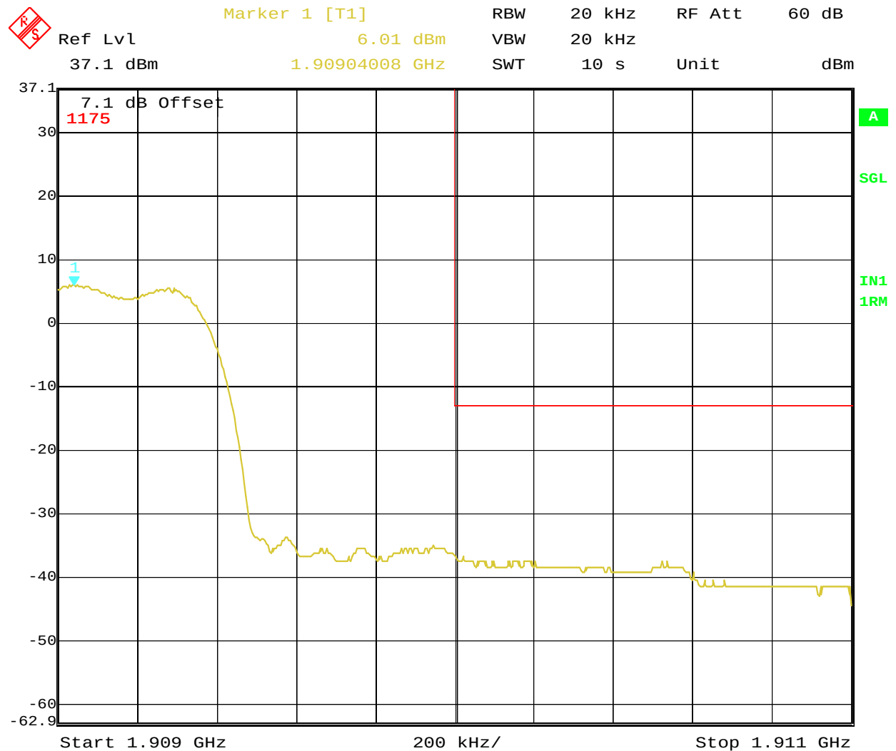
Figure 8-8: Emissions within 1 MHz of band edge, CDMA 1900 Channel 1175
