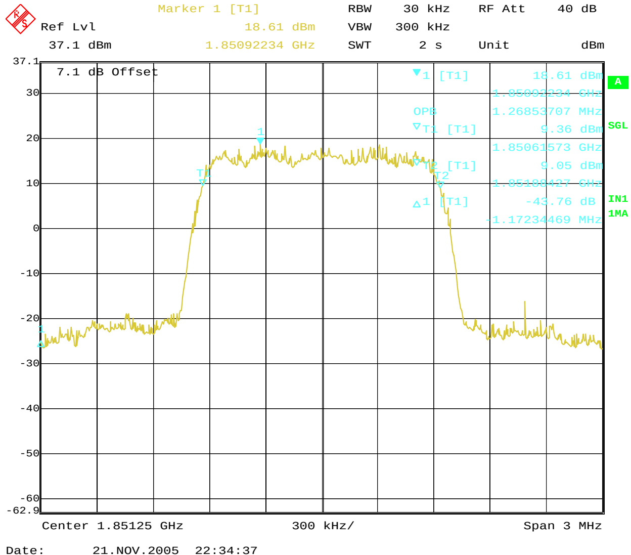
Figure 7-4: Occupied Bandwidth – PCS Channel 25
