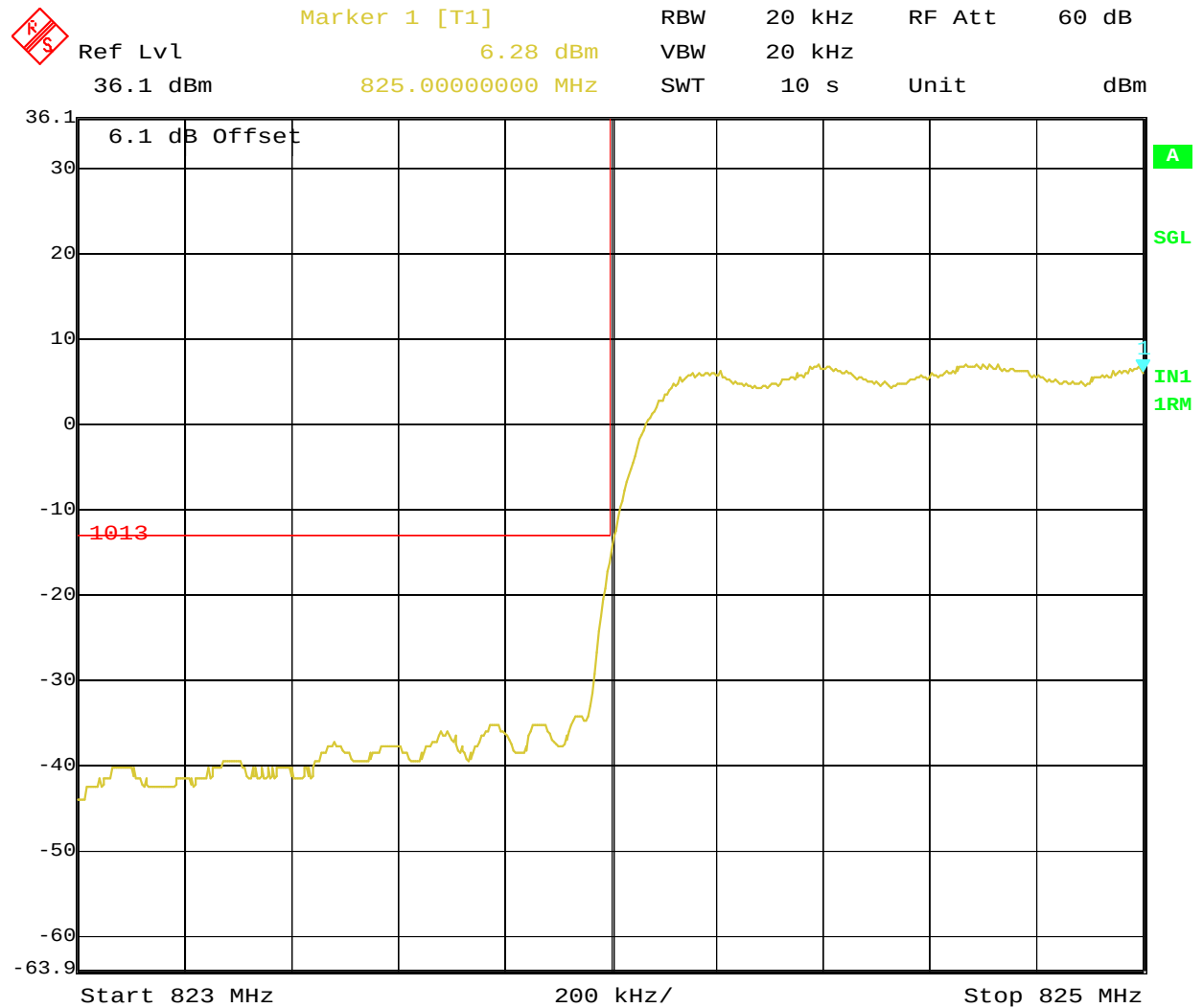
Figure 8-5: Emissions within 1 MHz of band edge, CDMA 800 Channel 1013
