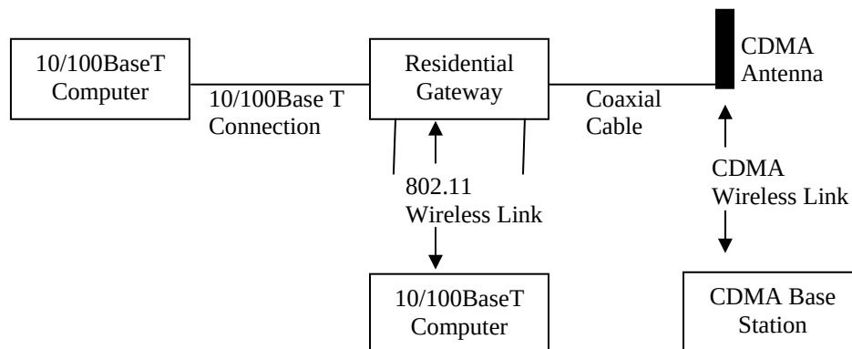
Figure 1-1: Radiated Test Configuration
