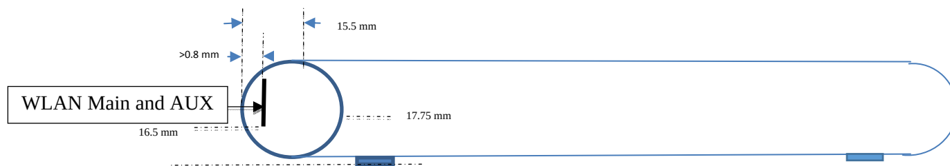
Side View of Antenna Placement in EUT
