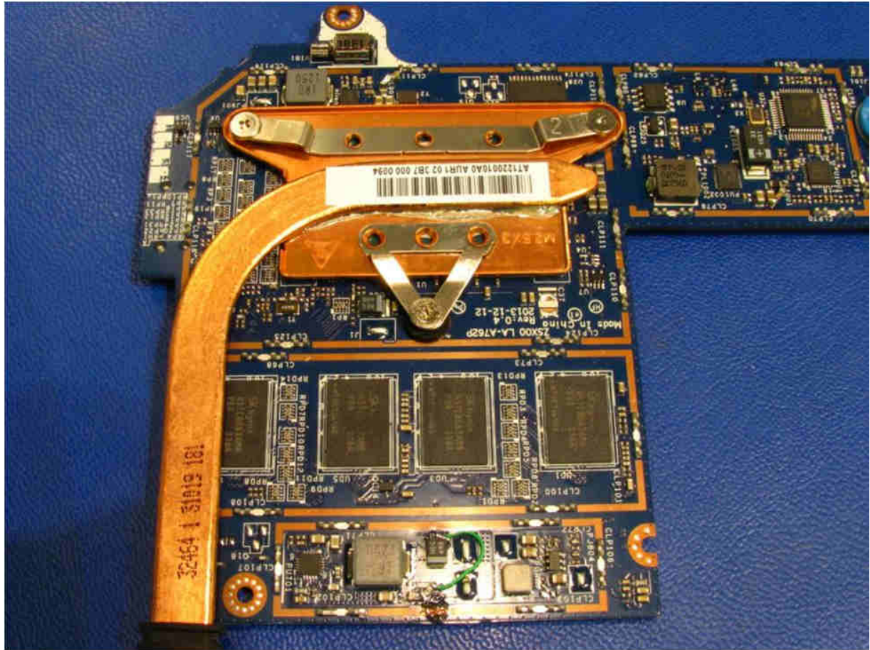
Main PCB Back Side – Right End of PCB without RF Shields
