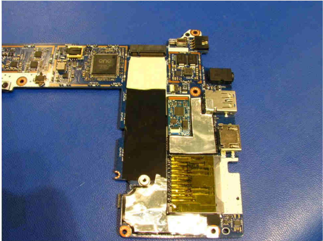
Main PCB Back Side – Left End of PCB without RF Shields
