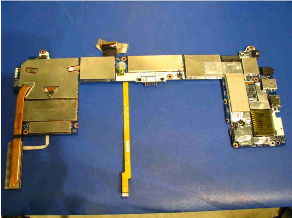
Main PCB Back Side with RF Shields
