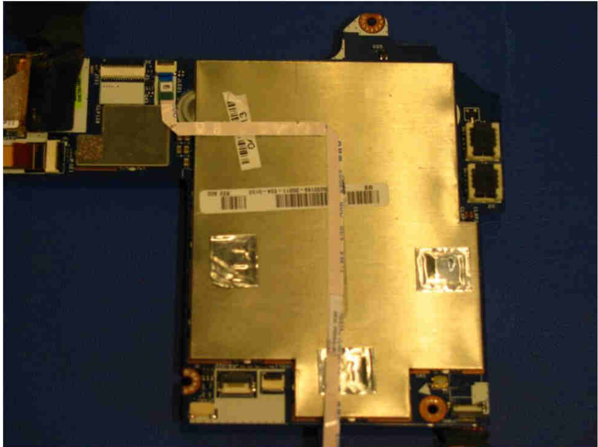
Main PCB Front Side – Right End of PCB with RF Shields
