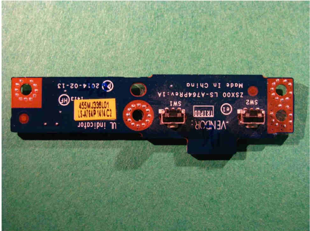
Volume Up / Down Button PCB Back Side
