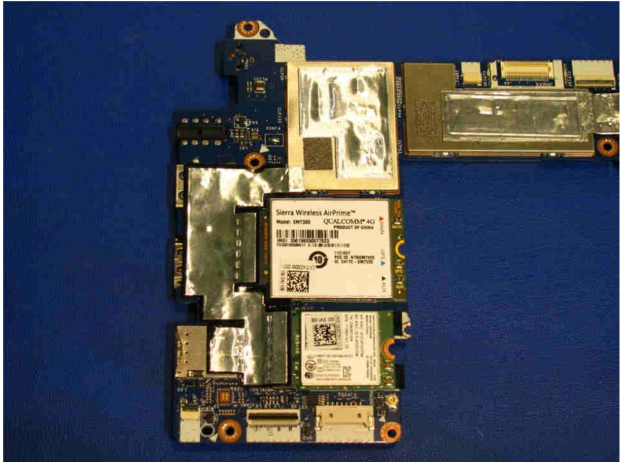
Main PCB Front Side – Left End of PCB with RF Shields
