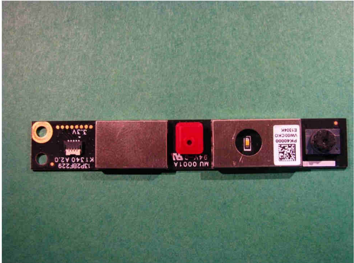
Ambient Light Sensor PCB Front Side
