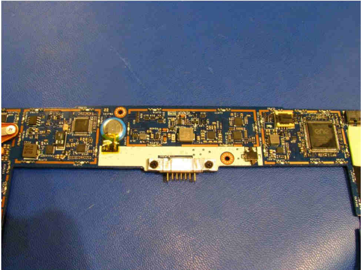
Main PCB Back Side – Center of PCB without RF Shields
