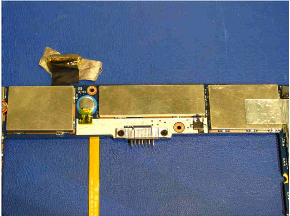
Main PCB Back Side – Center of PCB with RF Shields
