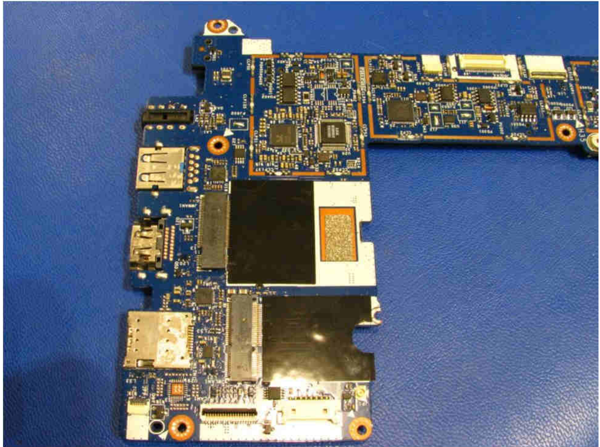
Main PCB Front Side – Left End of PCB without RF Shields
