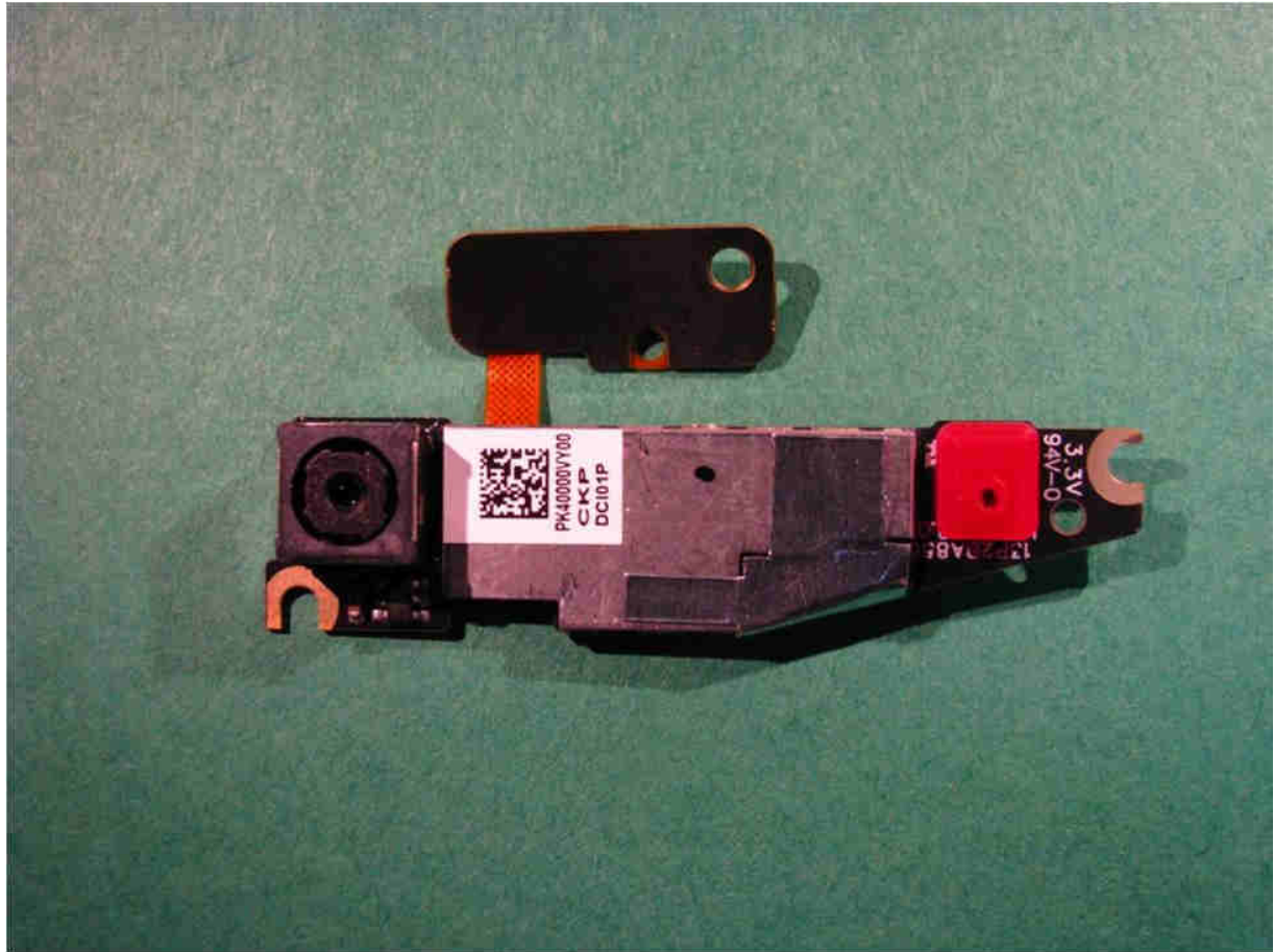
Camera PCB Front Side & Flash LED Back Side
