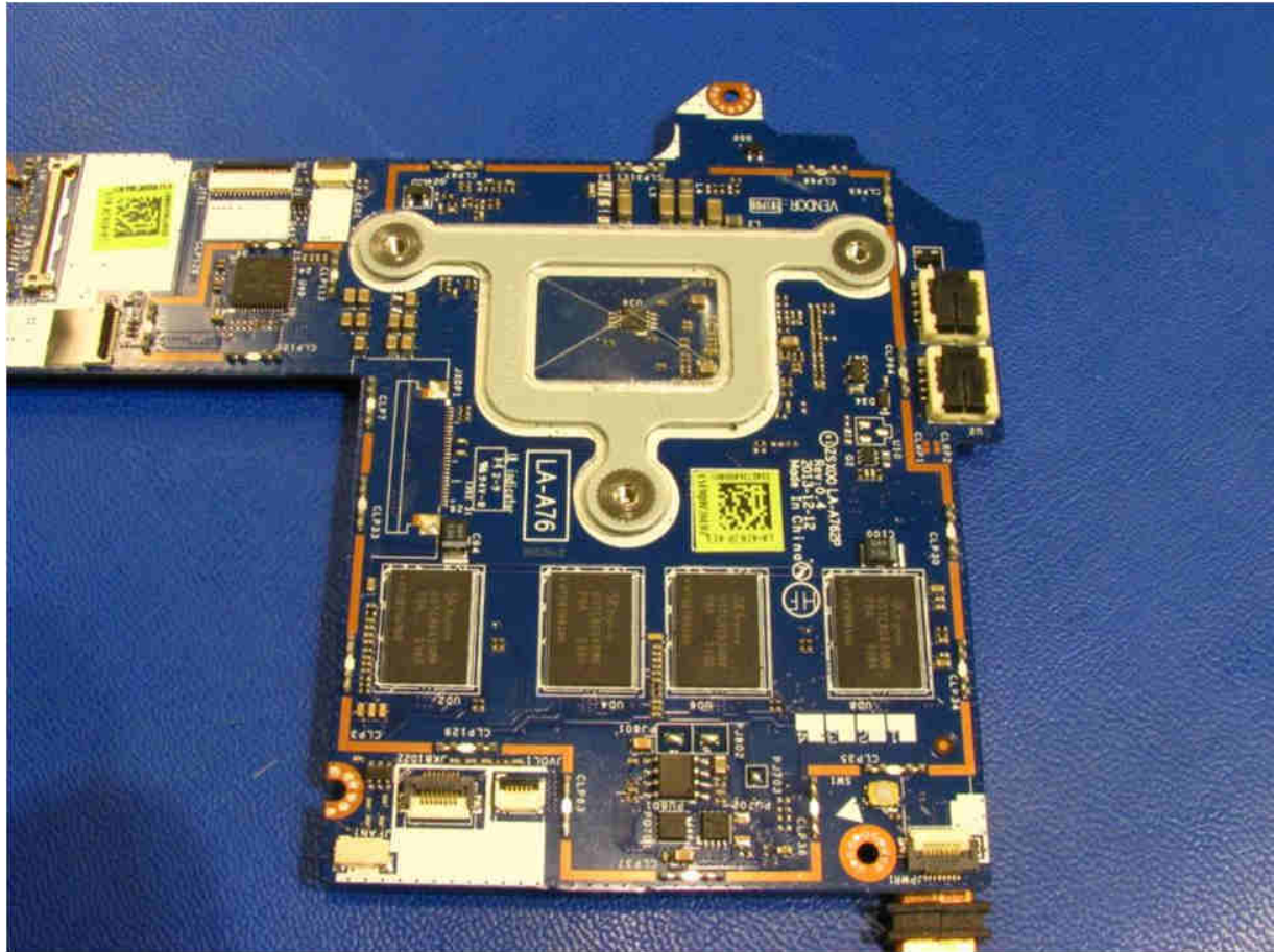
Main PCB Front Side – Right End of PCB without RF Shields
