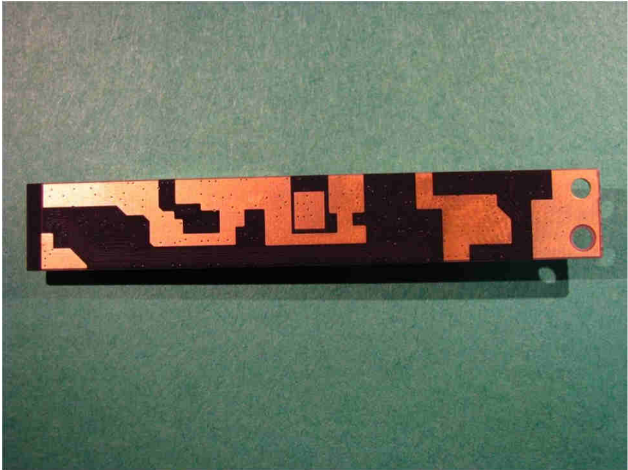
Ambient Light Sensor PCB Back Side
