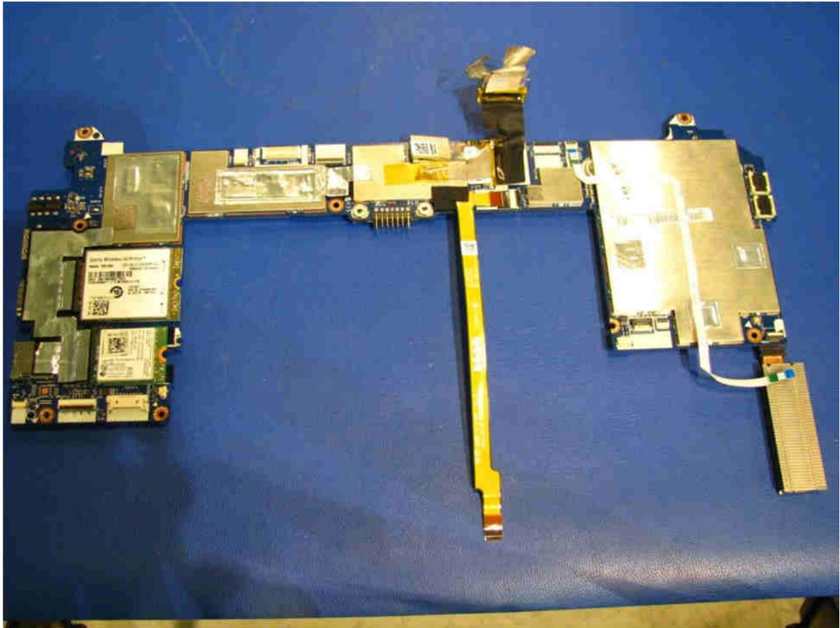
Main PCB Front Side with RF Shields
