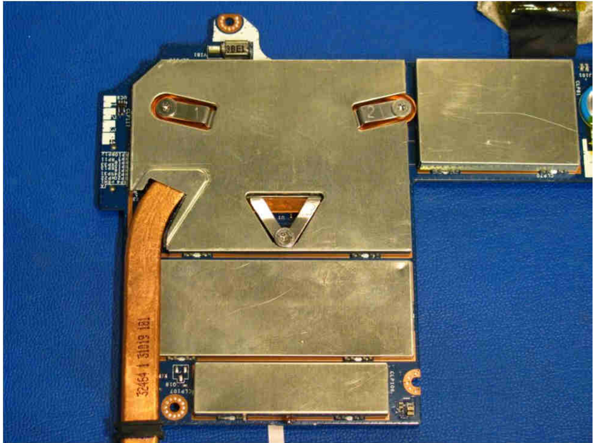
Main PCB Back Side – Right End of PCB with RF Shields
