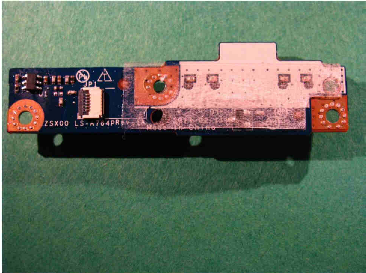
Volume Up / Down Button PCB Front Side
