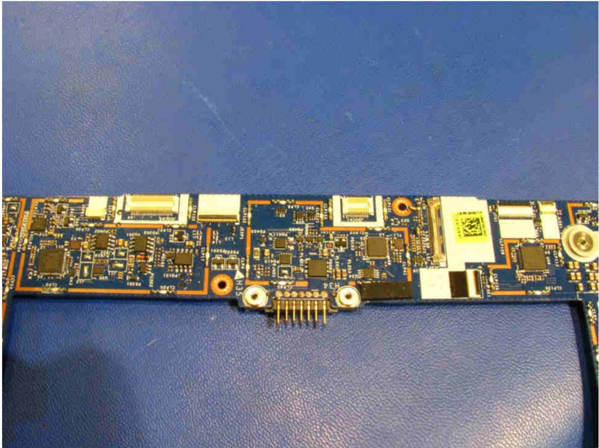
Main PCB Front Side – Center of PCB without RF Shields
