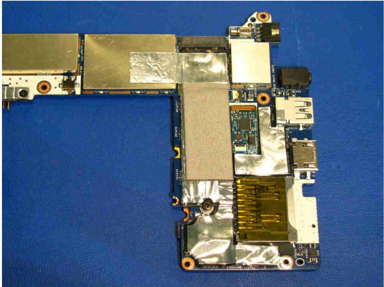
Main PCB Back Side – Left End of PCB with RF Shields
