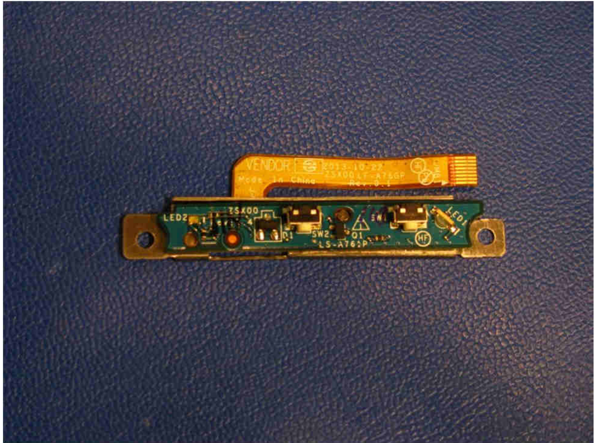
Power Button PCB Back Side
