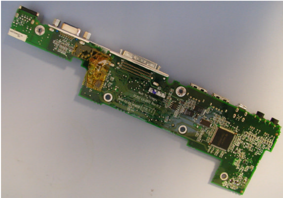
IO Board
